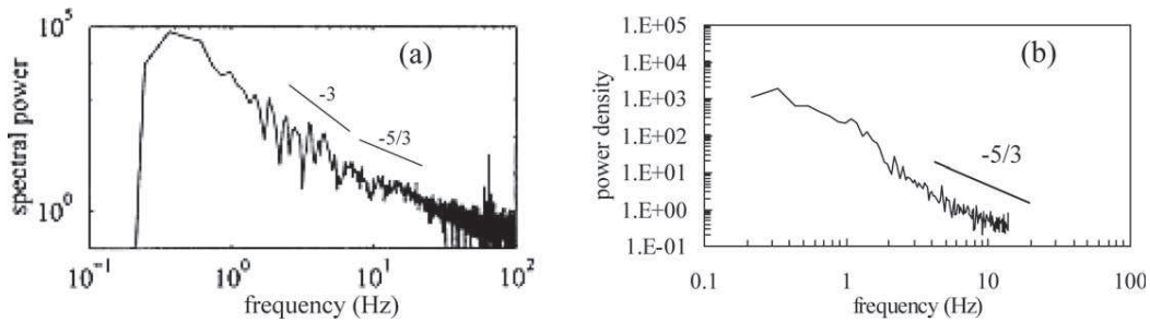
Figure 14. Solid fraction power spectrum \phi_p = 0.56 (nylon beads). (a) Experiments (b) Numerical.
