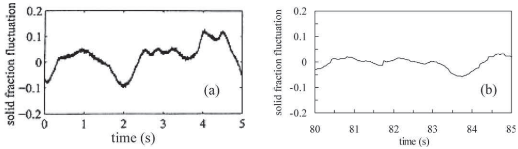
Figure 13. Solid fraction fluctuations \phi_p = 0.56 (nylon beads). (a) Experiments (b) Numerical.
