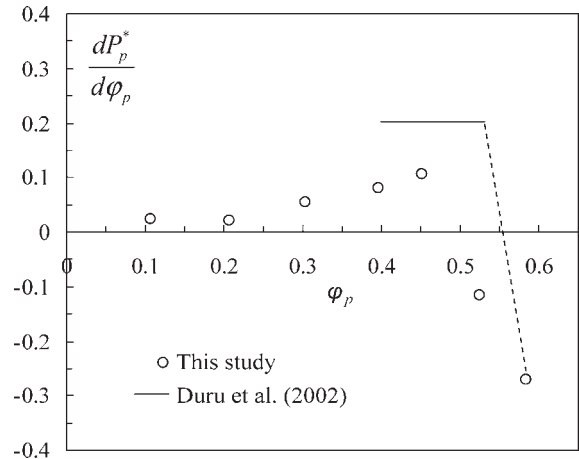
Figure 10. Reduced elasticity as a function of \phi_p .
