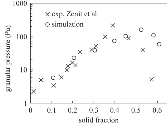
Figure 1. Granular pressure averaged in the bed as a function of averaged solid fraction for steel beads.
