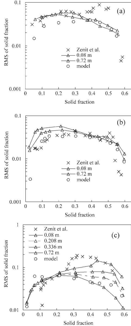
Figure 19. RMS of solid fraction as a function of \varphi_p . (a) nylon beads (b) glass beads (c) steel beads.
