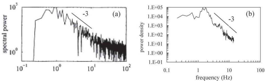
Figure 18. Solid fraction power spectrum \phi_p = 0.47 for steel beads. (a) Experiments (b) Numerical.
