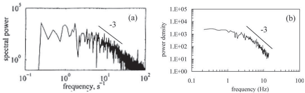
Figure 16. Solid fraction power spectrum \phi_p = 0.11 (steel beads). (a) Experiments (b) Numerical.
