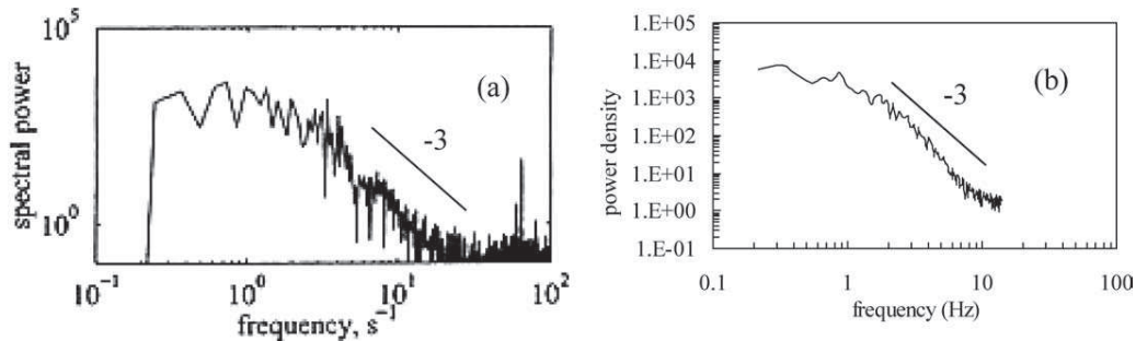
Figure 12. Solid fraction power spectrum \phi_p = 0.11 (nylon beads).
