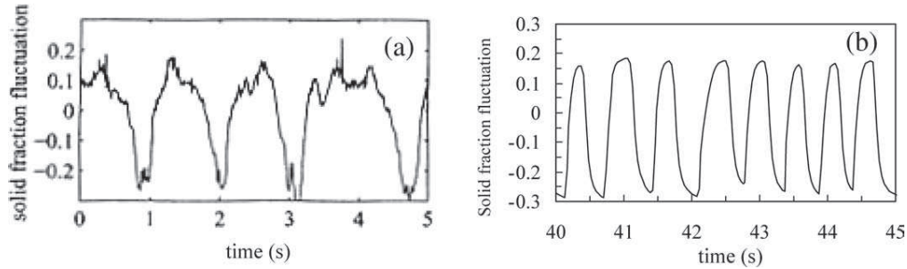
Figure 17. Solid fraction fluctuations \phi_p = 0.47 for steel beads. (a) Experiments (b) Numerical.
