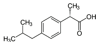
Fig. 1 – Ibuprofen molecular structure.
