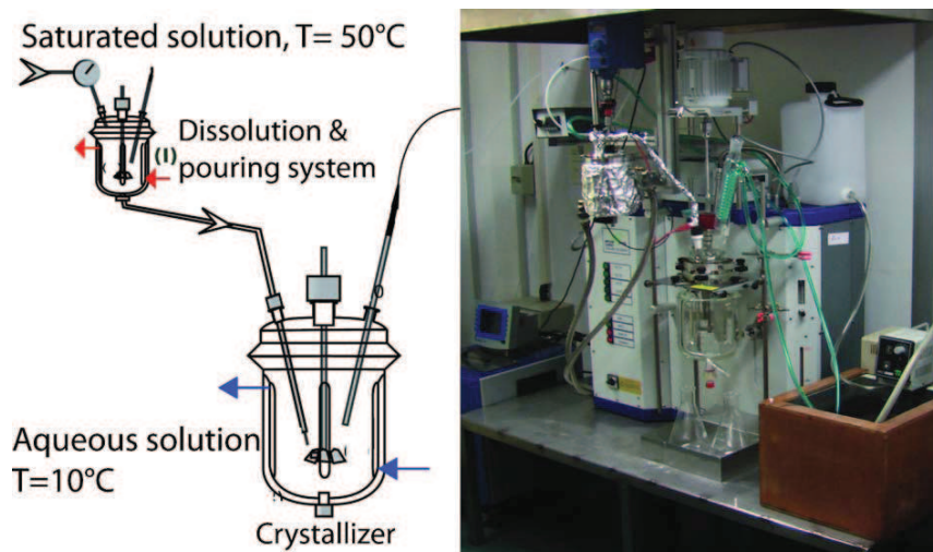
Fig. 2 – Spherical crystallization process experimental setup.
