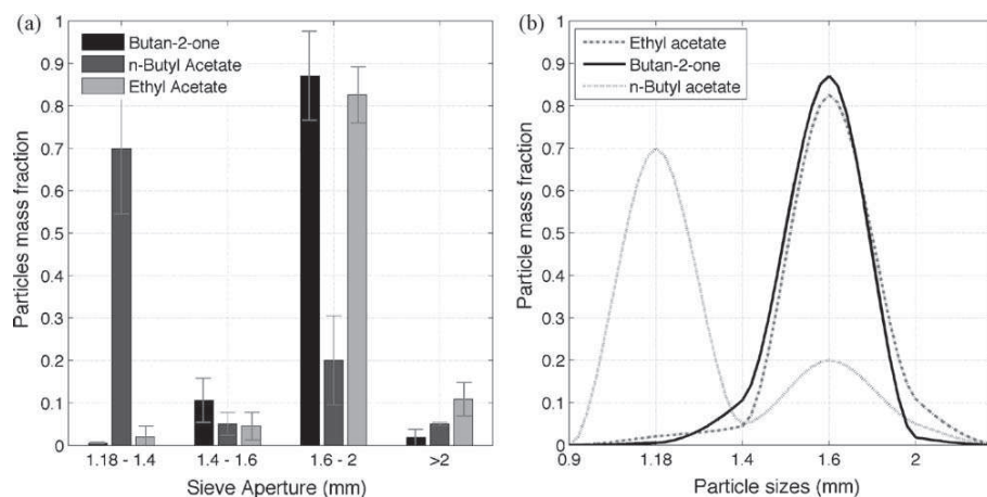
Fig. 8 – Particle sizes distribution for different crystallization solvents. (a) Experimental size distribution; (b) interpolated sizes distribution.
