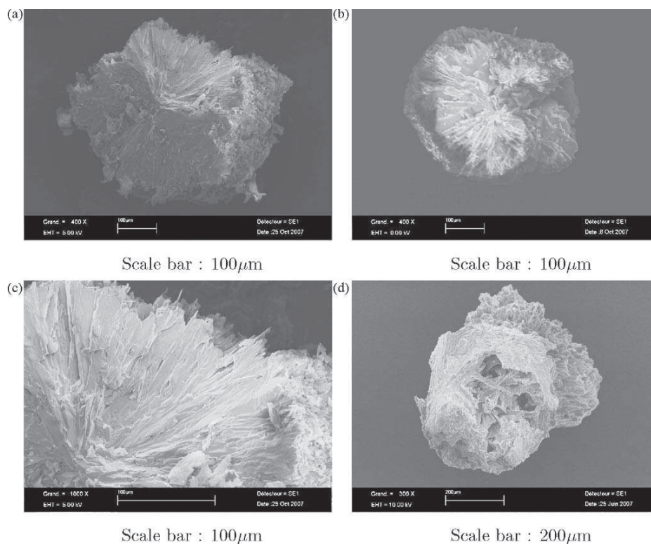
Fig. 4 – Microphotograph of broken primary particles.
