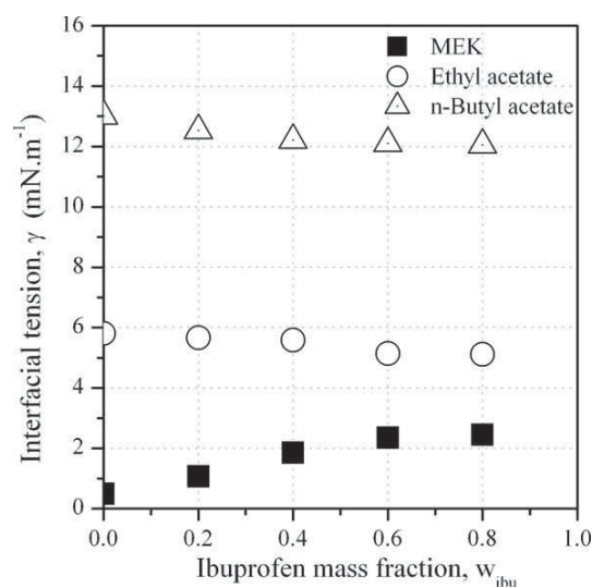
Fig. 7 – Organic phase/water interfacial tension as a function of the mass fraction of ibuprofen introduced in the solvent.
