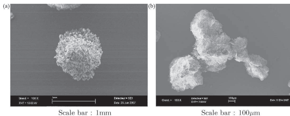
Fig. 3 – Microphotograph particles obtained in ethyl acetate/water system. (a) Spherical primary particles; (b) secondary agglomerates.
