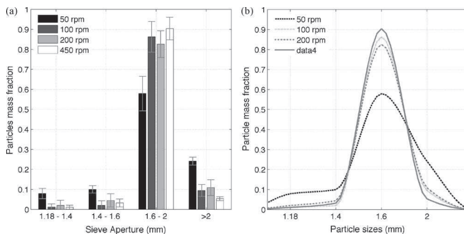
Fig. 5 – Particle sizes distribution for different stirring rates in ethyl acetate/water system. (a) Experimental size distribution; (b) interpolated sizes distribution.
