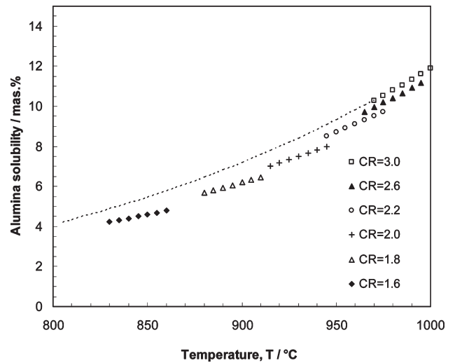
Figure 6. Solubility of alumina versus temperature at constant overheating in the system \text{Na}_3\text{AlF}_6 – \text{AlF}_3 , for various \text{CR} . Temperature range is comprised between the liquidus temperature T_{\text{liq}} and T_{\text{liq}} + 50^\circ\text{C} (calculated from ref 3).
