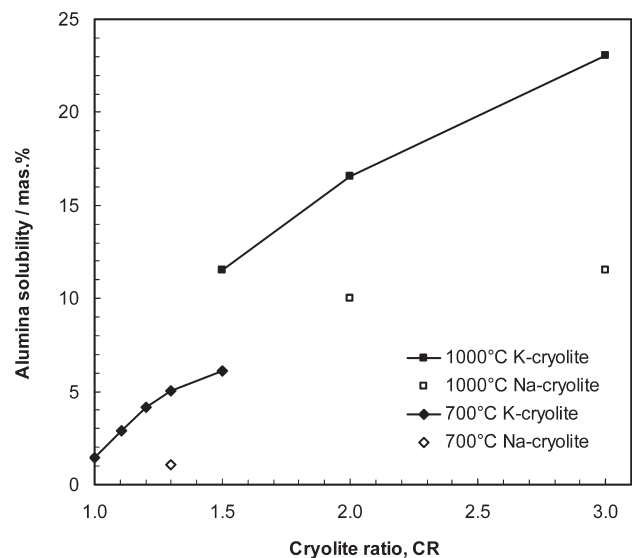
Figure 15. Alumina solubility in K–cryolite mixtures versus CR at 700 °C (Yang 27 ) and 1000 °C (Robert 7 ). Comparison to alumina solubility in Na–cryolite mixtures.
