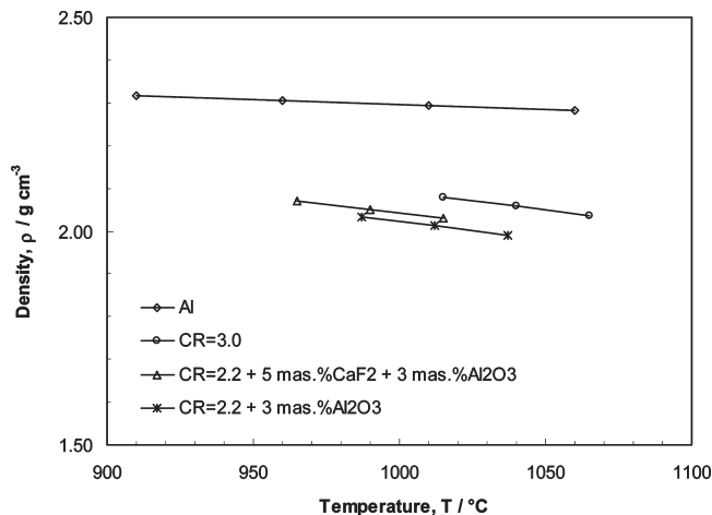
Figure 4. Influence of temperature and composition on the density of cryolite melts. 1,13,14
