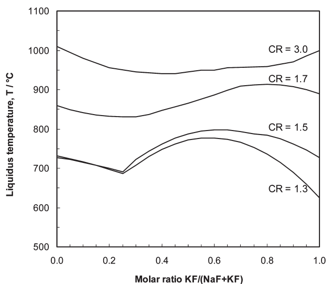
Figure 21. Liquidus temperature in the NaF-KF-AlF 3 system with different CR (from Apisarov 34 and Grjothem 35 ).
