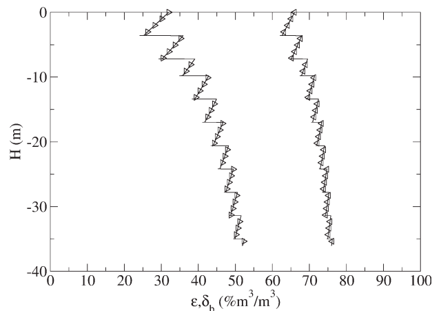
Figure 3. Model prediction of the industrial standpipe reported by Matsen 19 : local bubble phase fraction, \delta_b ( \blacktriangleright ) and local suspension porosity, \varepsilon ( \blacktriangleleft ).
