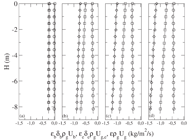
Figure 12. Model prediction of the small-scale standpipe reported by Masten 19 : local gas mass flux through bubble phase, \delta_b \varepsilon_b \rho_g U_b ( \circ ), the emulsion phase, \delta_e \varepsilon_e \rho_g U_{g,e} ( \square ), and total value, \varepsilon \rho_g U_g ( \diamond ).
