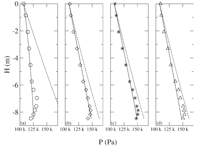
Figure 9. Comparison between the vertical profile of pressure predicted by the model (with friction: —, without friction: ---) and the small-scale make-up data of Srivastava (symbols).
