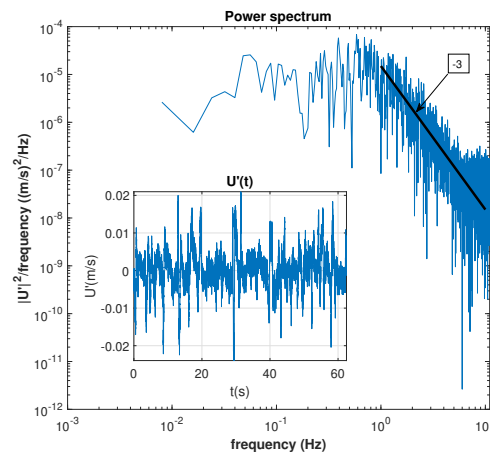
Figure 3: Power spectrum and U' vs t for the point drawn on Fig. 2a.
