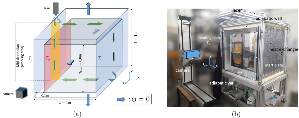
Figure 1: a): 3D configuration with working area b): experimental apparatus
