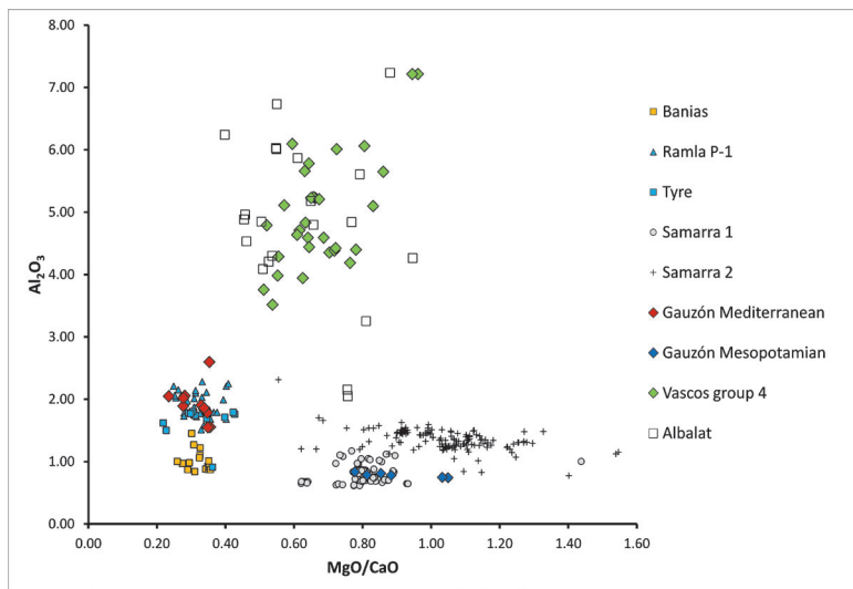
Fig. 3: Aluminium oxide compared with magnesium to calcium ratios of plant ash glass groups from Spain (Albalat, Vascos and Gauzon) in comparison with glasses from Mesopotamia (Samarra) and the Levant (Banias, Ramla and Tyre). Data source: Banias (FREESTONE, GORIN-ROSEN and HUGHES, 2000), Group P-1 of Ramla (Phelps, 2018), Tyre (FREESTONE 2002), Groups 1 and 2 of Samarra (SCHIBILLE et al., 2018), Gauzón (DE JUAN et al., 2018a), Group 4 of Vascos (DE JUAN and SCHIBILLE, 2017) and Albalat (publicacion in preparation).
