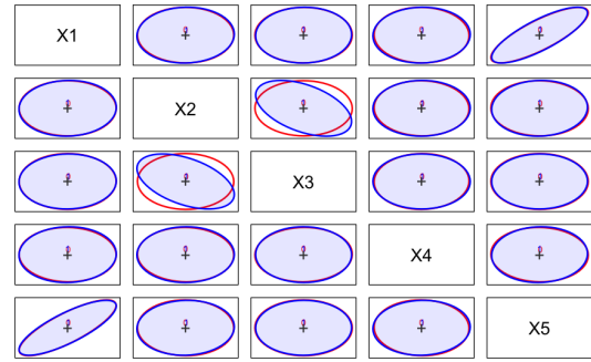
(b) Situation B - Centered pairwise data ellipses
