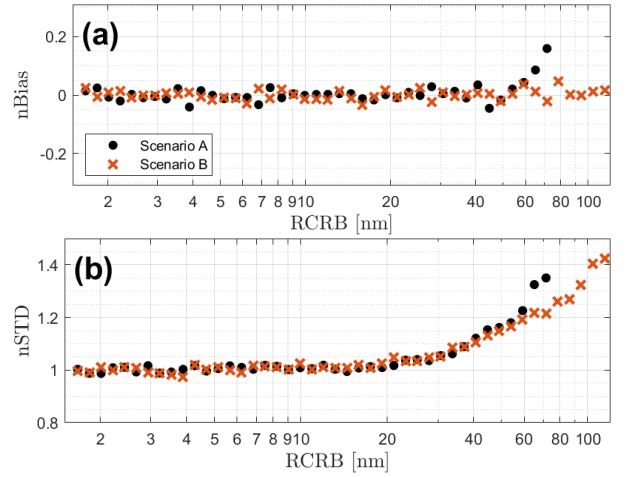
Fig. 3. Estimation properties of the MLE when the fluorescent emitter is in-focus and at the corner of a pixel for (a) the normalized bias (nBias), (b) the normalized standard deviation (nSTD), as a function of the RCRB for Scenario A (black dots) and B (red crosses). The simulation parameters are given in Fig. 2 except for \theta_0 = (5, 5) \mu\text{m} .
