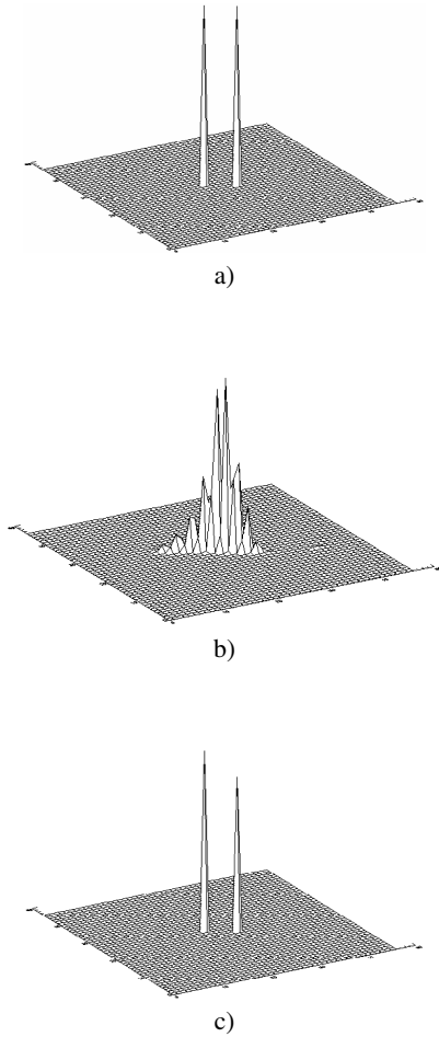
Fig. 4. Example of application of the two-step algorithm. The object is a binary consisting of two stars with angular separation \frac{1}{4}\lambda/B ( B = maximum baseline of LBT) and with the same magnitude m = 12 ; three interferometric noisy images are generated by convolving the object with the PSFs with an average Strehl ratio of 66% and are deconvolved by means of the PSFs with an average Strehl ratio of 77% (see Fig. 3): a) the original object; b) the restored object obtained after Step 1; c) the restored object obtained after Step 2.
