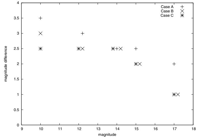
Fig. 5. Behaviour of the maximum magnitude difference \Delta m_0 which can be detected as a function of the magnitude m of the main component – monolithic case. For the sake of clarity coincident points are represented with a small horizontal shift.
