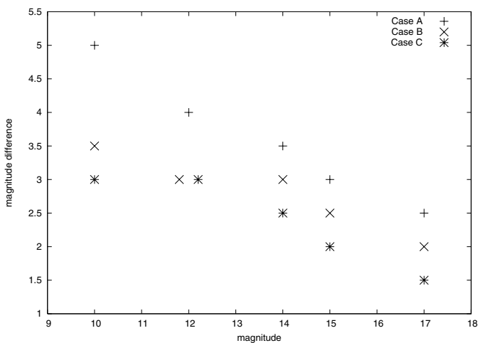
Fig. 6. Behaviour of the maximum magnitude difference limit \Delta m which can be detected as a function of the magnitude m of the main component – interferometric case. For the sake of clarity coincident points are represented with a small horizontal shift.
