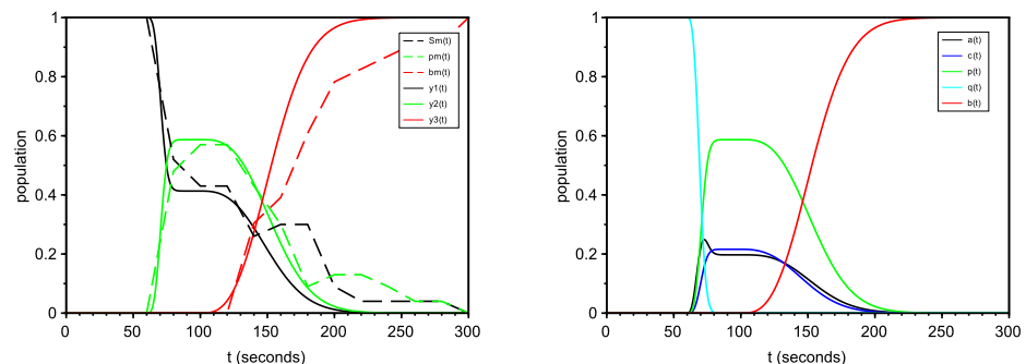
Figure 9. (Left): Representation of real data S_m, p_m, b_m , and the output trajectories: densities of the control ( y_1 ), panic ( y_2 ), and everyday ( y_3 ) behavior after the catastrophe. (Right): Simulations of a, p, c, b, q with the parameters obtained from the genetic algorithm.
