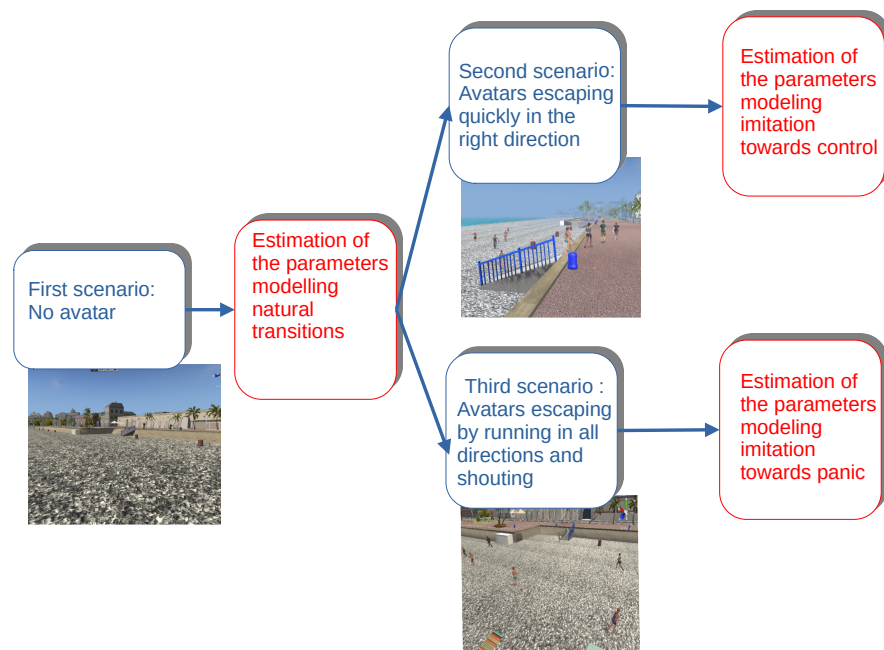
Figure 8. Diagram summarizing the steps of the identification of the model parameters. The natural transitions will be first estimated from the first scenario. Then, imitation processes will be identified from the second and third scenarios.
