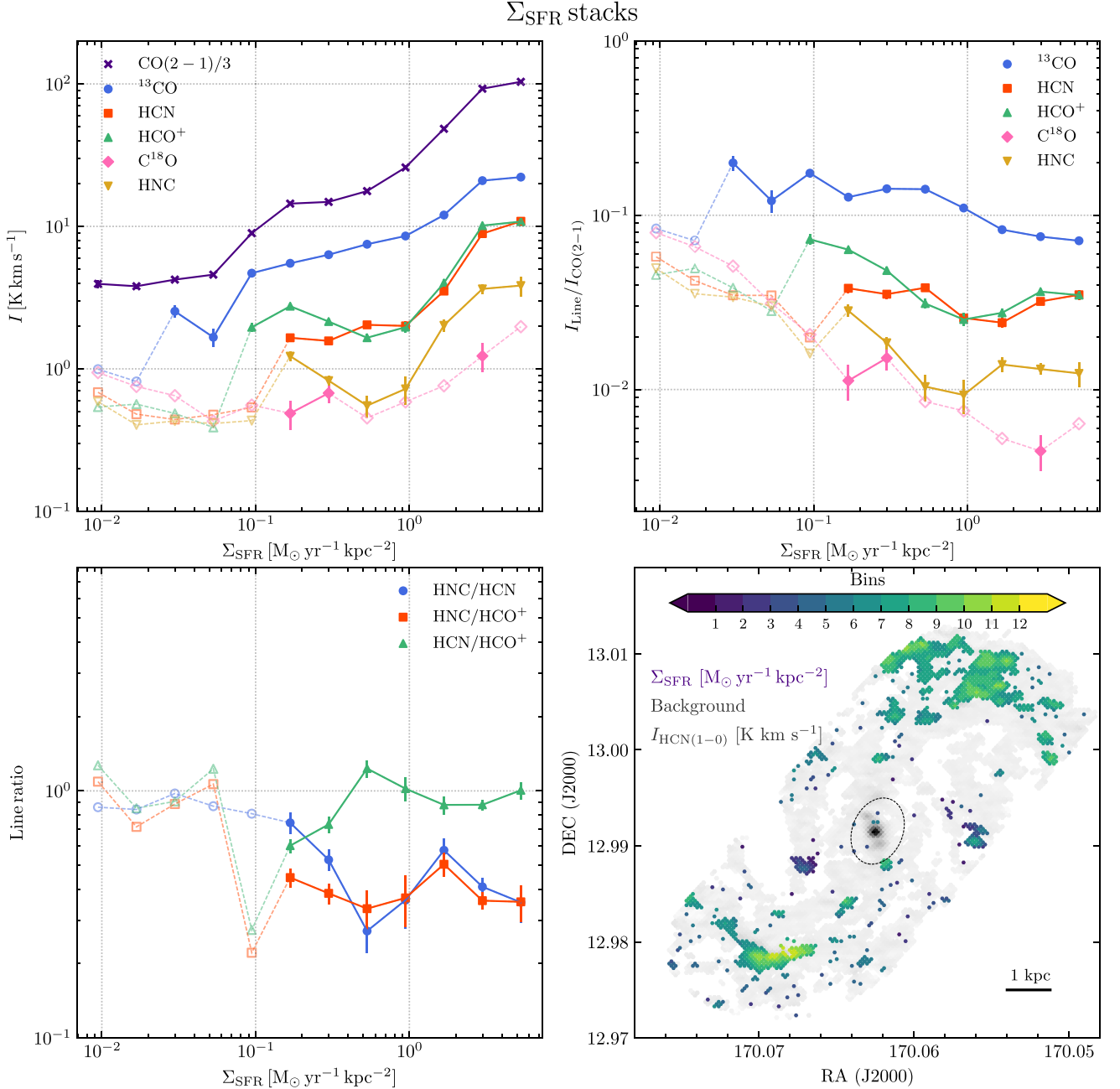
Figure 5. Same as Fig. 3, but for stacks by \Sigma_{\text{SFR}} . We stack data points from regions where star formation is traced by \text{H}\alpha emission (Section 2.3). We exclude the centre (region within the circle with radius of \sim 600 pc) where \text{H}\alpha emission may not exclusively trace recent star formation. We also show the HCN integrated intensity map in grey in the bottom right-hand panel.
