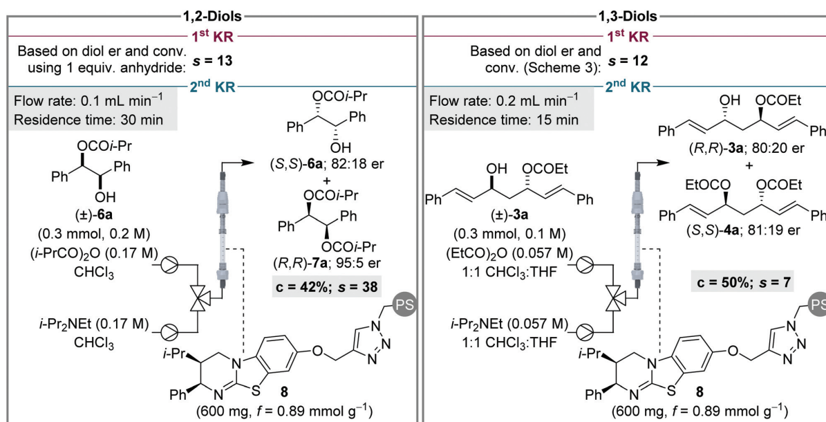
Scheme 6 Assessment and comparison of s values for individual KR steps for the sequential KR of both (±)-1,2- and (±)-1,3-diols.
