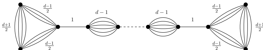
Figure 1: The padded paddle graph
