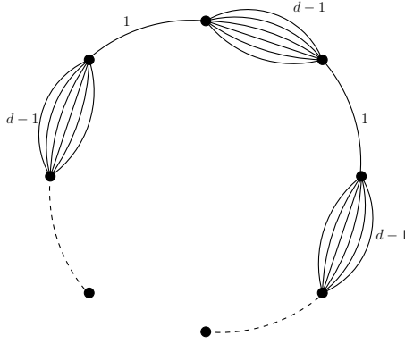
Figure 2: The padded cycle graph
