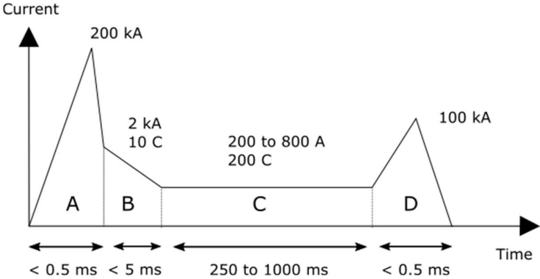
Fig.1. The standardized lightning current waveforms
