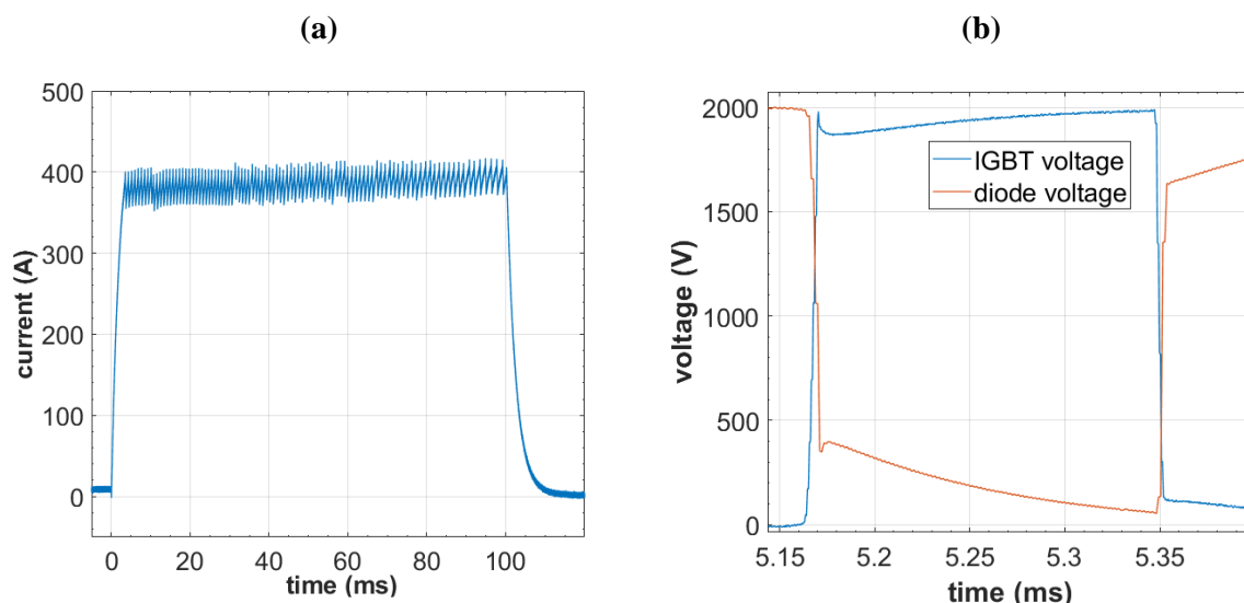
FIG 12. Current (a) and voltages (b) waveforms of Buck configuration for a 4 \Omega load resistance
