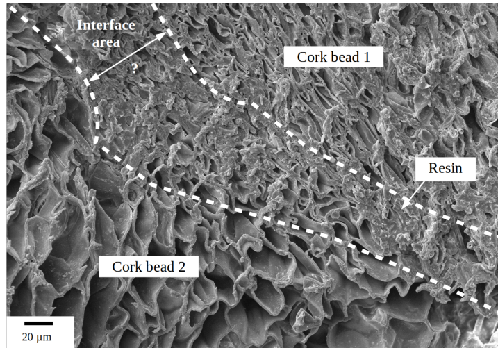
(a) Intergranular interphases in the unreinforced foam [21].
