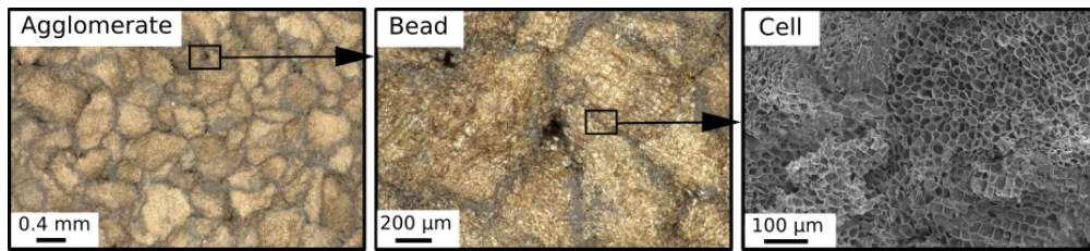
(b) Agglomerated cork observed at several magnifications.
