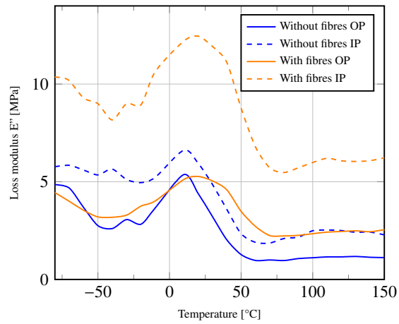
(b) Loss modulus E'' .
