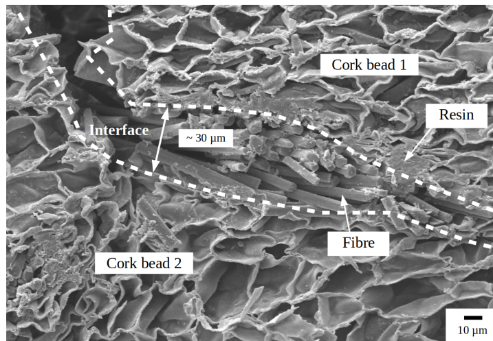
(b) Intergranular interphases in the reinforced foam.
