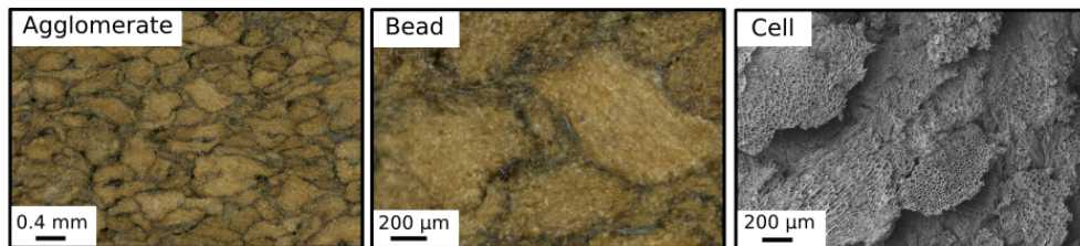
(c) Reinforced agglomerated cork observed at several magnifications.
