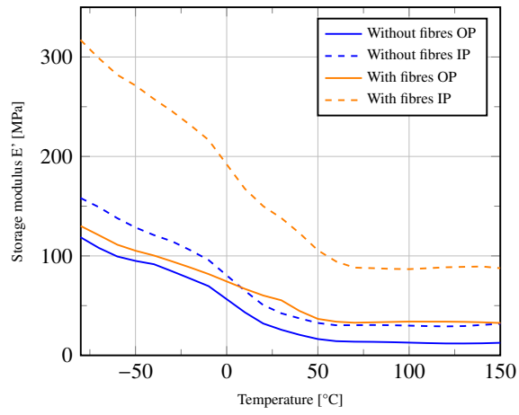
(a) Storage modulus E' .
