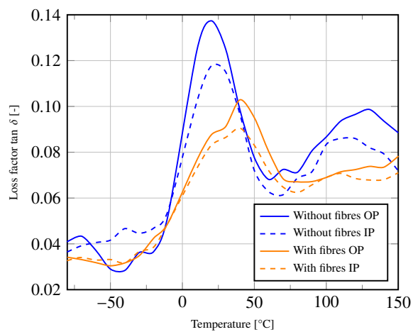
(c) Loss factor \tan \delta .
