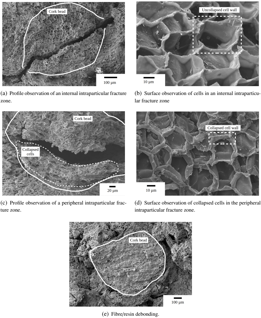
Figure 9: Fracture surface and profile observed with a SEM of multiscale foams after mode I fracture tests.
