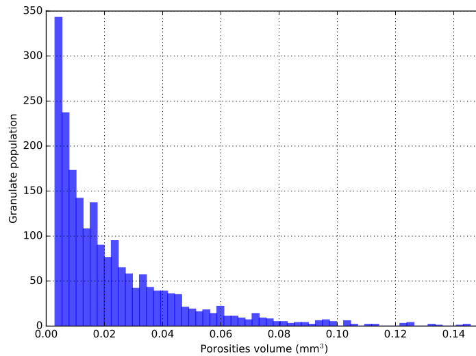
Figure 14: Results from computed tomography. Distribution of porosities volume in a cork agglomerate obtained by uni-axial compression.
