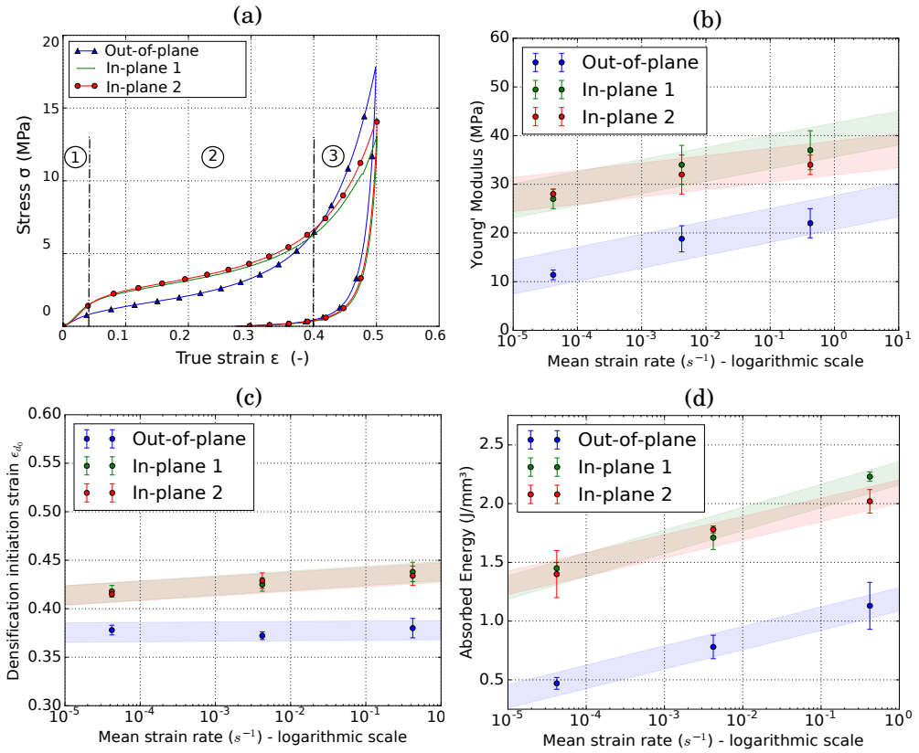
Figure 19: Results of the compressive loadings. (a) A typical experimental compression curve of agglomerated cork tested in the 3 directions. (b) Young's modulus of cork agglomerates depending on the cross-head speed and the direction. (c) Densification initiation strain \epsilon=\epsilon_{d_0} of cork agglomerates depending on the mean strain rate and the direction of sollicitation. (d) Absorbed energy at \epsilon=\epsilon_{d_0} of cork agglomerates depending on the mean strain rate and the direction of sollicitation.
