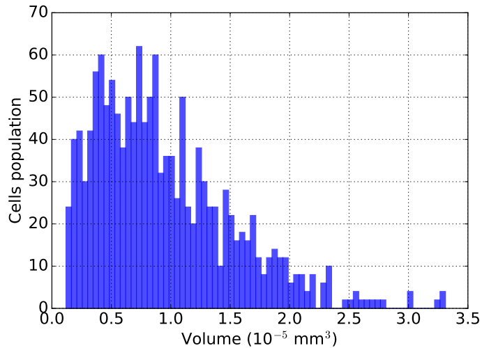
Figure 17: Results from computed tomography. Cork cells volume distribution of cork agglomerate obtained by uni-axial compression.
