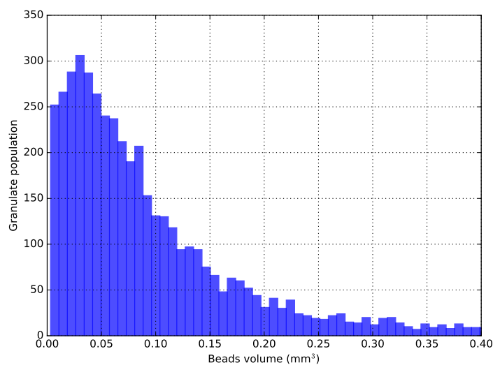
Figure 13: Results from computed tomography. Distribution of beads volume in a cork agglomerate obtained by uni-axial compression.
