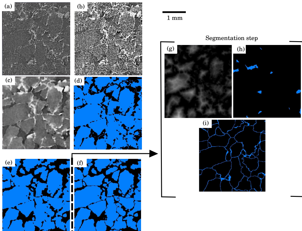
Figure 5: Post-treatment process of X-ray microtomography data. a) Raw picture. b) Histogram equalisation. c) Median filter. d) Thresholding. e) Opening. f) Segmentation. Steps of the segmentation operation . g) Inversed Chamfer distance map. h) Marker selectionned thanks to H-maxima technique. i) Watershed lines obtained with a marker-based segmentation.
