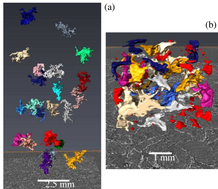
Figure 15: 3D reconstruction of porosities between cork beads. a) 40 biggest porosities in the whole sample. b) All the porosities in a subvolume.
