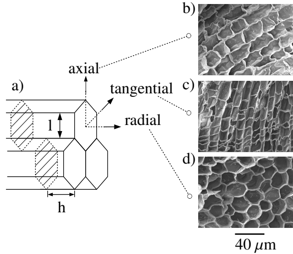
Figure 1: a) Natural cellular disposition of cork. b) Axial direction. c) Tangential direction. d) Radial direction. SEM Pictures.
