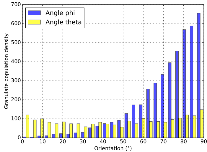
Figure 9: Orientation of cork granulates obtained through X-ray microtomography.
