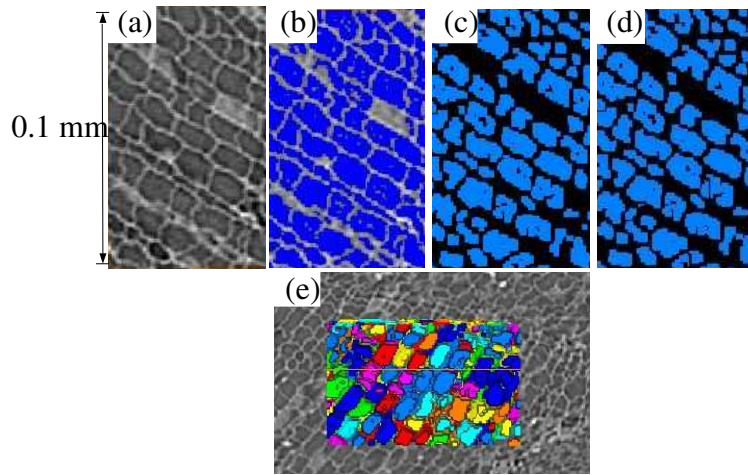
Figure 6: Process to obtain 3D information on cork cells. a) Raw image. b) Thresholding. c) Opening. d) Separation. e) Volume rendering
