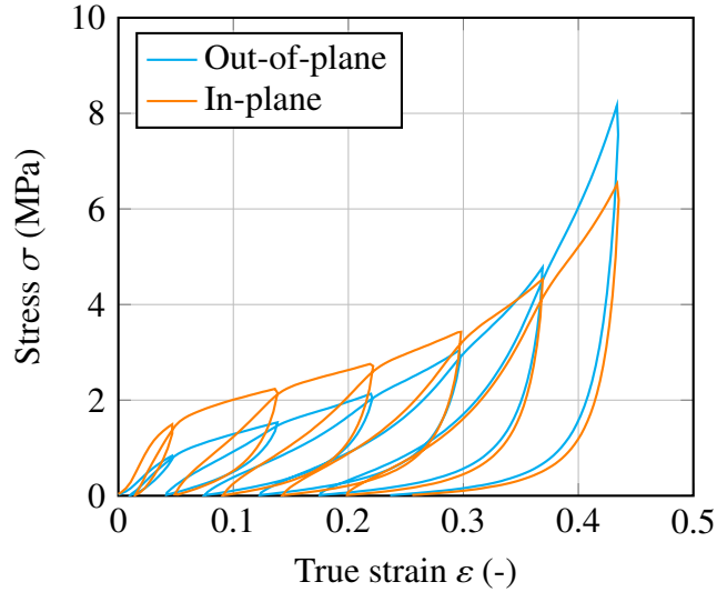
Figure 20: Experimental cyclic strain-stress curve of agglomerated cork in different directions.
