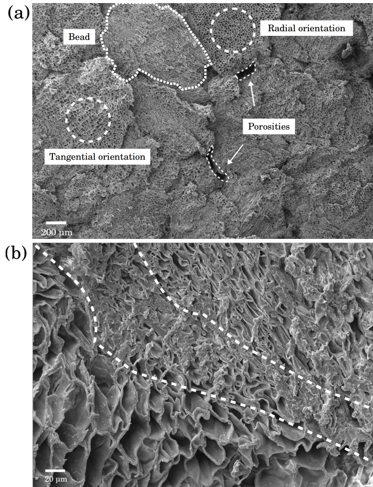
Figure 12: SEM pictures of cork agglomerate at different scales. (a) Intricate microstructure. Random cells orientation encircled. Porosities highlighted by arrows. (b) Interface between two cork granulates. Approximative delimitation by dotted lines.
