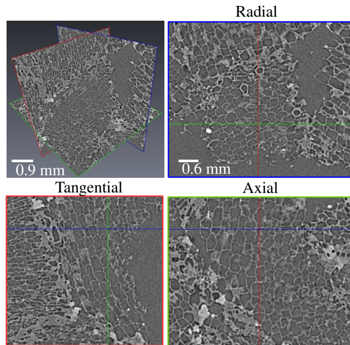
Figure 16: Orthoslices of a subvolume obtained by computed tomography. The three main directions of cork cells are presented (radial, tangential and axial).
