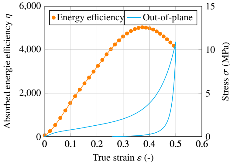
Figure 7: Experimental curve showing the energy absorption efficiency depending on the strain for agglomerated cork compressed in the out-of-plane direction at 5 \text{ mm min}^{-1}
