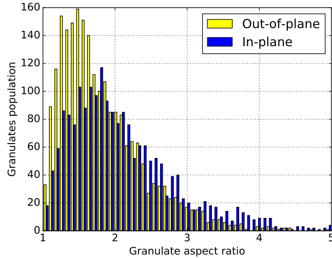
Figure 10: Results of picture analysis. Distribution of the granulates aspect ratio.
