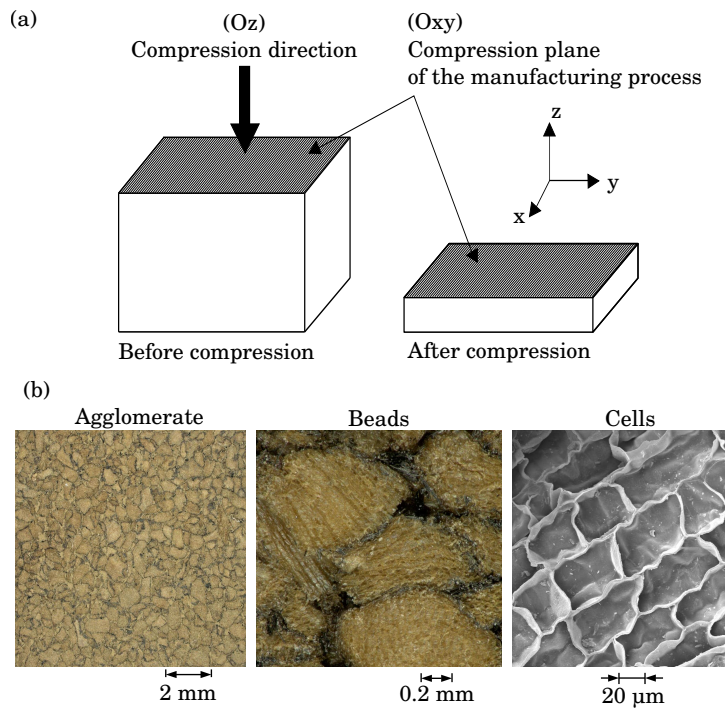
Figure 2: Agglomerated cork: a multi-scale material influenced by the manufacturing process. (a) Orientations resulting from the process. (b) Different observation scales demonstrating the multi-scale structure of agglomerated cork. At the agglomerate and bead scales, pictures are taken with a light microscope. Cells scale is illustrated with a SEM image of cork cells observed in the axial direction
