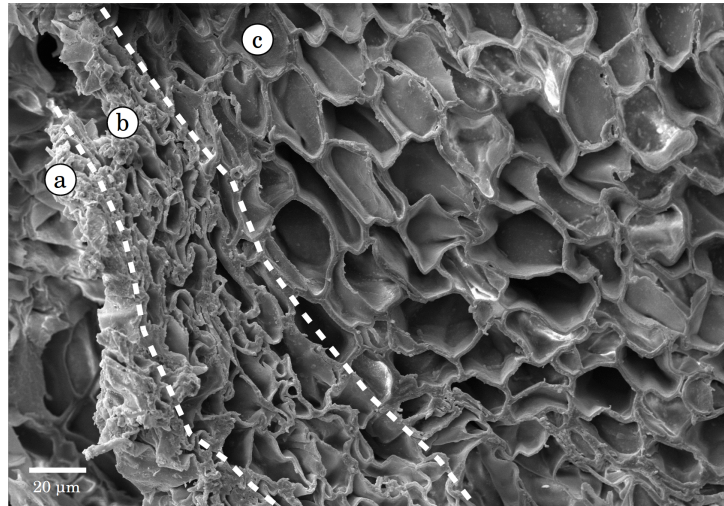
Figure 18: SEM picture of the periphery of a cork bead (a) Interface. (b) Cork cell distortion in the vicinity of the interface. (c) Undamaged cells.
