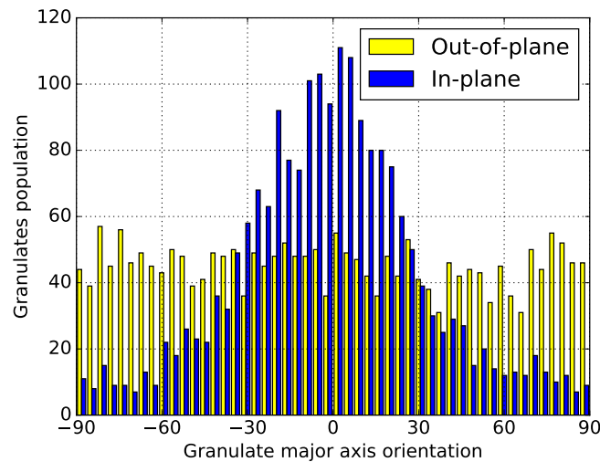
Figure 8: Results from surface observation. Histograms of the granulates major orientation in cork agglomerates.
