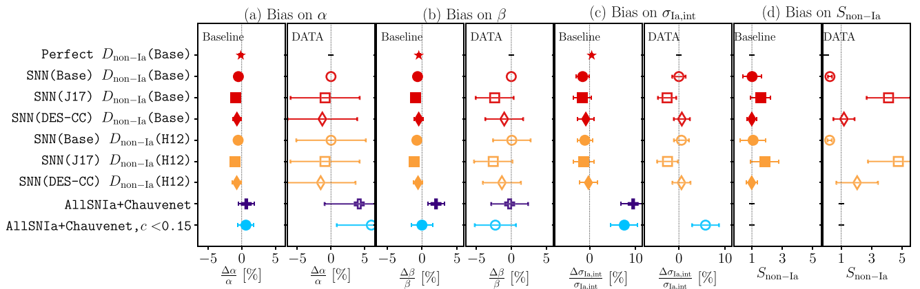
Figure 12. Relative differences in the fitted nuisance parameters \alpha (panel a), \beta (panel b), and \sigma_{Ia,int} (panel c), and the deviation from one of the scaling parameter S_{non-Ia} (panel d). Each pair of panels presents the results for Baseline (left) and DES-SNSYR data (right). We compare different BBC configurations (see Table 9). The BBC fitting procedure does not return uncertainty on \sigma_{Ia,int} . Therefore, for both data and simulations the uncertainties on \sigma_{Ia,int} are estimated as the r.m.s. spread in \sigma_{Ia,int} measured from the 50 realizations of the Baseline simulation.
