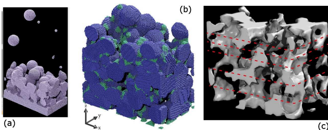
Figure 6. (a) MD simulation snapshot of the landing process employed to build the virtual film. (b) Rendering of the final virtual NP thin film. The Ag atoms composing big (set B) and small (set S) NPs are colored in blue and green, respectively, following the same color definitions as in Figure 3b. The average film thickness is 28.6 nm. (c) Void structure. The white 3D scaffold represents the voids between the deposited NPs. The cell base size for all panels is 35 \times 20 nm 2 . Panels (b,c) are adapted from ref. [25], further permission related to the material excerpted should be directed to the ACS.
