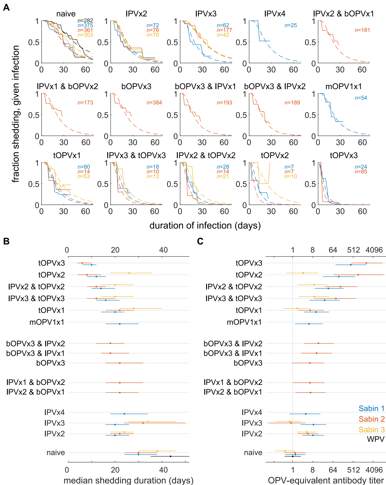
Fig 1. Effect of vaccination on shedding duration after OPV challenge and pre-challenge immunity. Labels describe vaccines received and number of doses (i.e., bOPVx2 and IPVx1: two doses of bOPV and one dose of IPV). (A) Sheddling duration after OPV challenge: shedding duration survival curves from aggregated trial data (solid lines) and maximum likelihood model fit (dashed) for each immunization schedule and poliovirus type.
