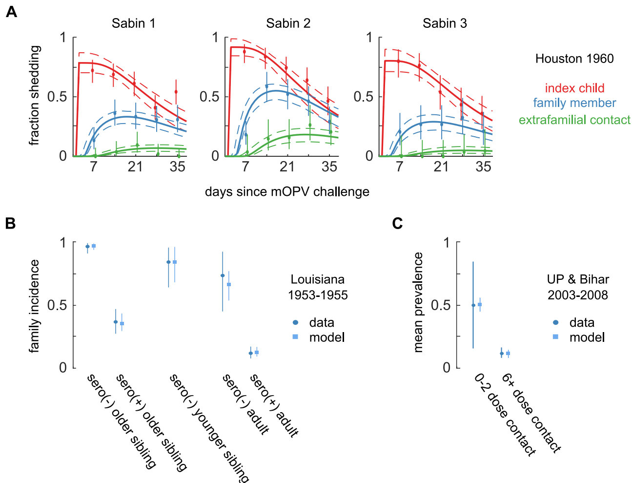
Fig 6. Transmission model calibration. Each study measured the amount of transmission from index persons in different ways. (A) Houston 1960: fraction of children under 5 years of age shedding each week after mOPV challenge to an index child and subsequent transmission. (Color by subject type; weekly data MLE and 95% CI, dot and whiskers; model MLE and 95% CI, lines). Eight free parameters are jointly identified across the nine calibration targets. (B) Louisiana 1953–1955: incidence in household contacts of index children naturally infected by WPV, measured by seroconversion approximately 30 days after the index child became infected. Three free parameters are jointly identified by the five calibration targets. (C) Uttar Pradesh and Bihar 2003–2008: mean prevalence of WPV in stool measured in household contacts after the onset of paralysis in index children. One free parameter is jointly identified by the two calibration targets. See S1 Text Fig C for additional information about model fit. CI, confidence interval; MLE, maximum likelihood estimate; mOPV, monovalent OPV; WPV, wild poliovirus.
