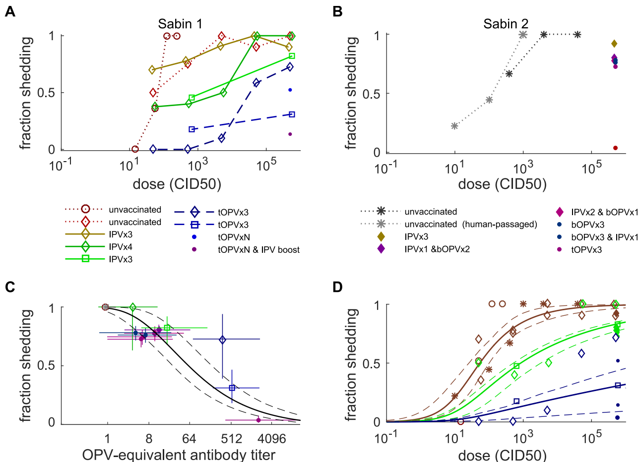
Fig 3. Oral susceptibility to infection after OPV challenge. (A) Fraction shedding after Sabin 1 oral challenge at different doses (color by trial arm, symbol by source study). (B) Fraction shedding after Sabin 2 oral challenge at different doses (color by trial arm, symbol by source study; data for doses \leq 10^3 CID50 are for human-passaged Sabin 2 isolated from stool 5 days after vaccination). (C) Fraction shedding at vaccine doses ( 10^{5-6} CID50) decreases with increasing OPV-equivalent antibody titer (color and symbols as in panels A–B; black lines are model MLE and 95% CI using S1 Text Eq E). (D) Beta-Poisson dose–response model MLE and 95% CI. Three model scenarios shown correspond to immunologically naive ( N_{Ab} = 1 , red), heterotypic bOPV and upper-bound IPV-only ( N_{Ab} = 8 , green), and typical tOPV or post-IPV-boosting ( N_{Ab} = 256 , blue). Data from panels A–B (symbols as above, colored by corresponding model scenario). bOPV, bivalent type 1 and 3 OPV; CI, confidence interval; CID50, the culture infectious dose that induces a cytopathic effect in 50% of infected cell or tissue cultures; IPV, inactivated polio vaccine; MLE, maximum likelihood estimate; OPV, oral polio vaccine; tOPV, trivalent OPV.
