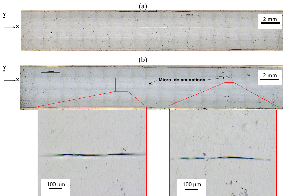
Fig. 12 Micrograph of the lengthwise section distribution of PA12 specimens: a after the FFF process, b after the fatigue test at r = 86\%
