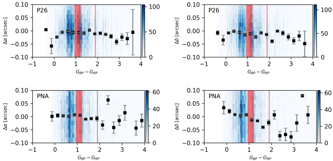
Fig. 9. Residuals for the Gaia stars as a function of color indices for the P26 and PNA satellite location areas. Red semi-transparent spans show the color indices of the main Saturnian satellites (the thin band at the G_{BP} - G_{RP} \approx 1.9 mag represents Titan's color). The (B-V) values for the Saturnian satellites were taken from Cruikshank (1978) . They were converted to the Gaia color system according to Jordi et al. (2010) . Color maps show the distribution of the differences over the color. Blue represents the number of differences in each bin, as indicated by the color bar.
