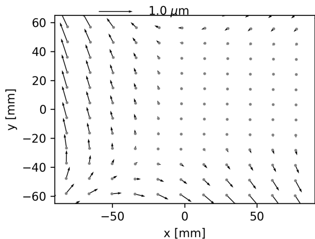
Fig. 6. Field distortion pattern for the NAROO-MDD template astronegative.
