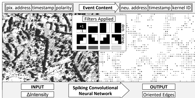
Fig. 2: CSNN results. Left: input data, B&W dots correspond to -1 & +1 event polarity respectively. Right: corresponding output data, round dots correspond to vertical and horizontal filters, triangles dots correspond to diagonal ones. Input data from [22].
