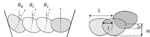
Figure 4 : Multipass welding with tilt parameters (left) and lateral and vertical remelting of a pass (right) [16].
