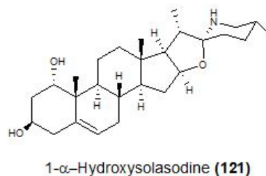
Figure 6: The chemical structures of 1 \alpha -Hydroxysolasodine (121).
