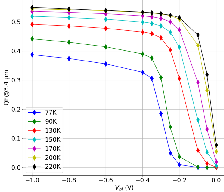
Figure 6: Evolution of the QE at 3.4 \mu\text{m} with the bias voltage in the temperature range 77K-220K. QE is for a frontside illuminated photodetector without antireflection coating.
