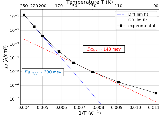
(a) Dark current density ( J_d ) as a function of applied bias V , (b) Arrhenius plot of the dark current density. Diffusion and measured at temperatures ranging from 90K to 325K. Generation-Recombination regimes are identified.
