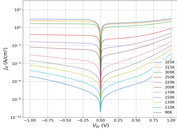
(a) Dark current density ( J_d ) as a function of applied bias V , (b) Arrhenius plot of the dark current density. Diffusion and measured at temperatures ranging from 90K to 325K. Generation-Recombination regimes are identified.
