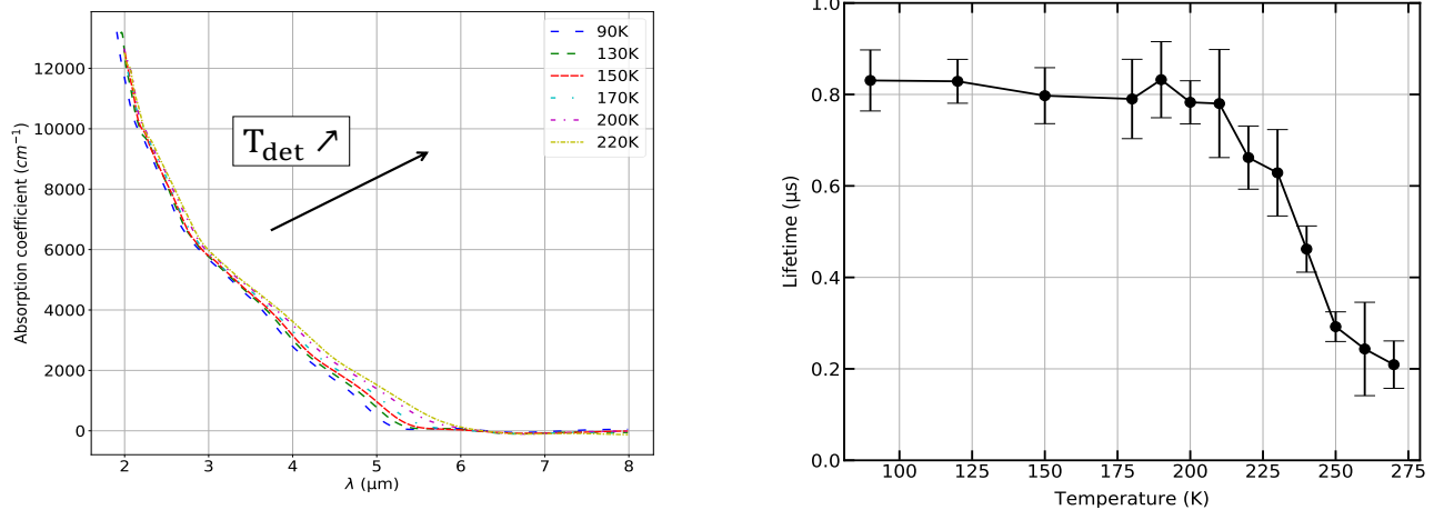
(a) Measured absorption coefficient of the InAs/InAsSb dedicated sample (Fig.1.b) for different temperatures. (b) Evolution of the measured minority carrier lifetime with temperature. Error bars are plotted to illustrate the measurement precision with the set-up
