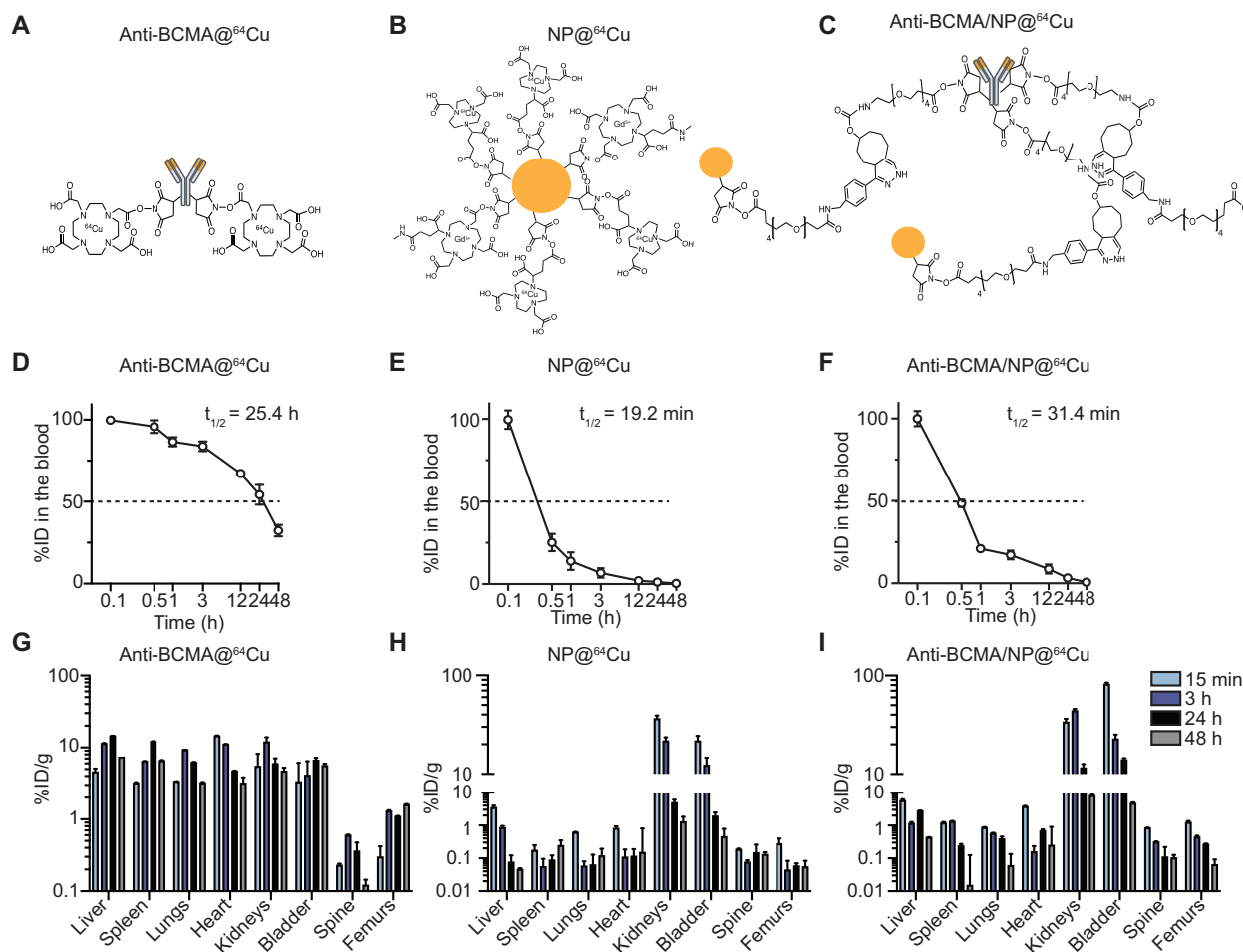
Figure 1. Design and pharmacokinetic profiles of the radioisotopes. A) Structures of the anti-BCMA@ ^{64}\text{Cu} immunoPET, B) untargeted NP@ ^{64}\text{Cu} , and C) anti-BCMA/NP@ ^{64}\text{Cu} immuno-nanoPET radiotracers. D) Pharmacokinetic profiles of anti-BCMA@ ^{64}\text{Cu} , E) NP@ ^{64}\text{Cu} , and F) anti-BCMA/NP@ ^{64}\text{Cu} in healthy BALB/c mice ( n = 5/\text{time point} ). G. Biodistribution data in the major organs over time in anti-BCMA@ ^{64}\text{Cu} , H. NP@ ^{64}\text{Cu} , and I) anti-BCMA/NP@ ^{64}\text{Cu} healthy BALB/c mice ( n = 5/\text{time point} ). All measurements were decay-corrected.
