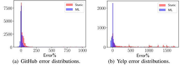
(a) GitHub error distributions.
