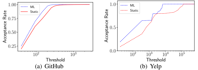
Fig. 5. Comparison of the acceptance rate against increasing threshold for the static analysis (red) and the ML approach (blue). The acceptance rate is computed as the number of queries whose sum of estimated complexity is below the threshold level divided by the number of sampled queries.
