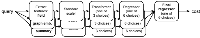
Fig. 3. Stacking ensemble overview.
