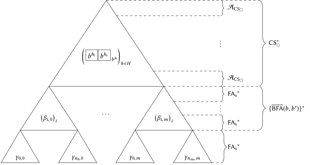
Fig. 13. The shape of the term is determined by the proof.
