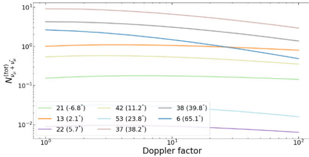
Figure 12. Stacked number of muon and antimuon neutrinos from flares with \Delta t < 30 d as a function of the Doppler factor for a few indicative sources (see inset legend; values within parentheses indicate declination angles). Other parameters used here are: B' = 10 G and \varepsilon_{\text{pk}} = 1 keV.
