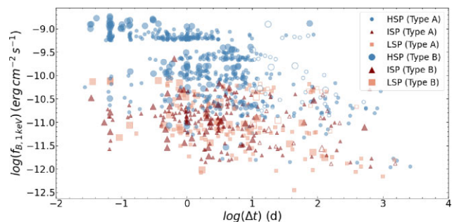
Figure 5. Block fluxes at 1 keV versus duration of blocks classified as flares of Types A and B. Different coloured symbols indicate the spectral blazar class (see inset legend). Open symbols indicate blocks with \Delta t > 10 d and only one flux measurement within this interval.
