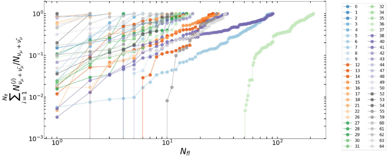
Figure 9. Cumulative number of muon and antimuon neutrino events expected from individual sources and N_{fl} X-ray flares with \Delta t < 30 d. Coloured symbols correspond to different sources, as indicated by their indices in the inset legend (for the source names see Table A1).
