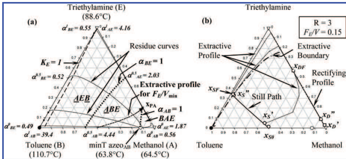
Figure 6. Methanol (A)–toluene (B) with triethylamine (E) 1.0-1b residue curve map and univolatility lines \alpha_{AB} and \alpha_{BE} . (a) and simulation results with F_E/V = 0.15 and R = 3 to recover A by extractive batch rectification (b).
