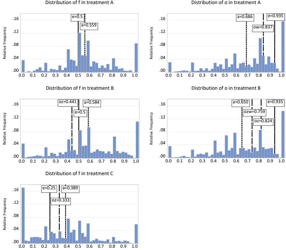
Figure 5: Distribution of weights assigned to x_{1,i} in the expectations of fundamental \theta and of others' action \bar{a}_{-i} ; e : equilibrium; a : realised average; oz : average optimum given individually realised z ; ozw : average optimum given individually realised z and \omega .
