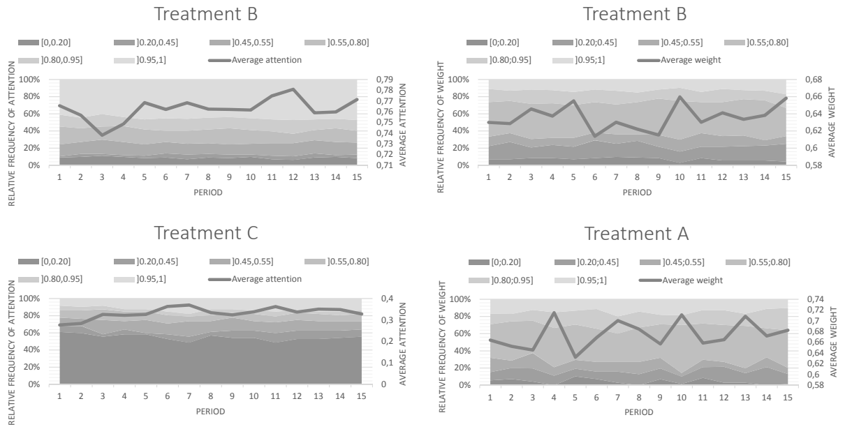
Figure 18: Convergence
