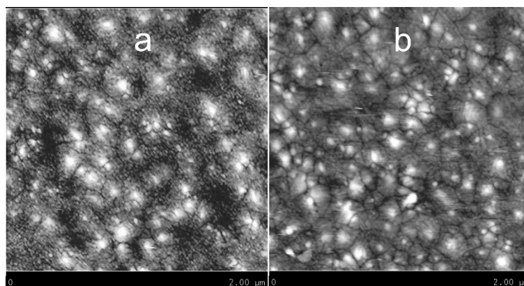
Figure 5. AFM images ( 2\ \mu\text{m} \times 2\ \mu\text{m} ) of \text{WO}_3 films annealed at 400\ ^\circ\text{C} (a) and 500\ ^\circ\text{C} (b) for 6 h, with a numerical treatment.
