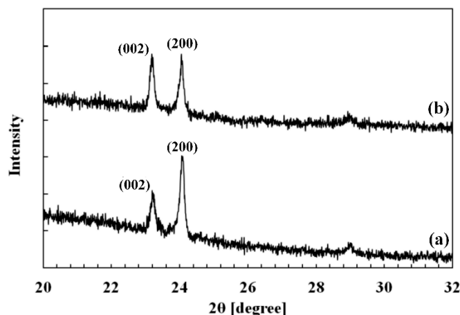
Figure 3. XRD spectra of \text{WO}_3 films annealed at 400 \text{ }^\circ\text{C} (a) and 500 \text{ }^\circ\text{C} (b) for 6 h in air. Peak indexations are related to either triclinic ( \delta\text{-WO}_3 ), monoclinic ( \gamma\text{-WO}_3 ), or orthorhombic ( \beta\text{-WO}_3 ) structures.
