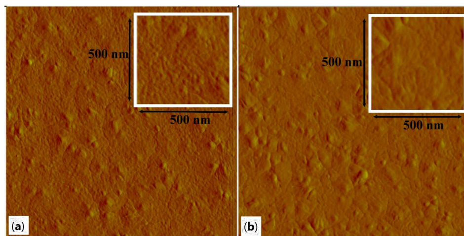
Figure 4. AFM images ( 2 \mu\text{m} \times 2 \mu\text{m} ) of WO_3 films annealed at 400 °C (a) and 500 °C (b) for 6 h. Insets: zoomed AFM images ( 500 \text{ nm} \times 500 \text{ nm} ).
