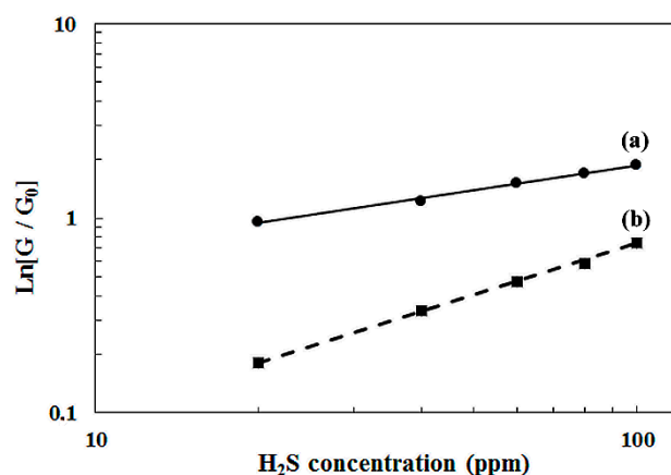
Figure 8. Sensitivity of sensor-400 (a) and sensor-500 (b) versus the \text{H}_2\text{S} concentration at 350 °C. The dots are experimental values. The lines are the fitting curves obtained with Equation (10).
