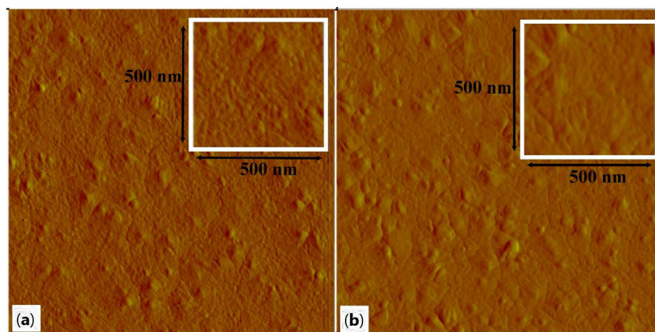
Figure 4. AFM images ( 2 \mu\text{m} \times 2 \mu\text{m} ) of WO_3 films annealed at 400 °C (a) and 500 °C (b) for 6 h. Insets: zoomed AFM images ( 500 \text{ nm} \times 500 \text{ nm} ).
