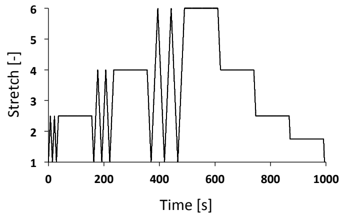
(b) Tests #2 and #3b: with relaxation phases
