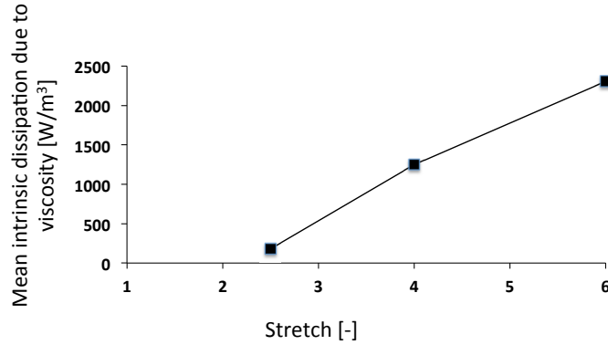
Figure 9: Mean intrinsic dissipation ( \tilde{D}_{int} ) due to viscosity plotted versus stretch. \tilde{D}_{int} is evaluated from the mechanically and thermally stabilized cycles of Test #1
