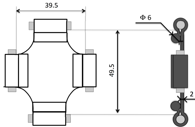
Figure 4: Specimen geometry for the biaxial test (dimensions in mm)
