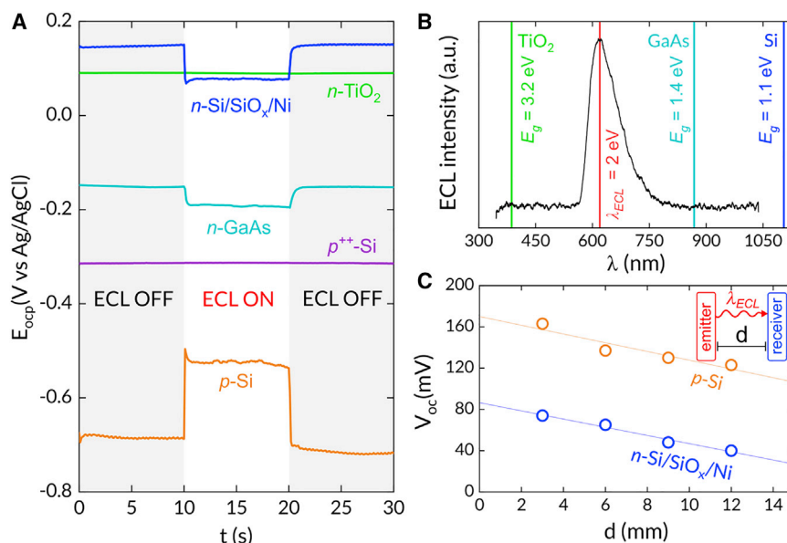
Figure 3. ECL-induced photovoltages
