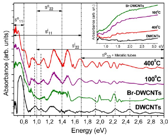
Figure 6. Optical absorption spectra for pristine and brominated DWCNTs and the brominated samples annealed in vacuum at 100 and 400 °C background corrected and scaled for better visibility. The insert shows the spectra without background correction. Dashed lines indicate peaks whose intensity or position was strongly modified by bromination.
