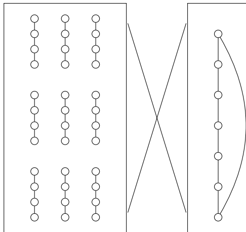
Figure 2: Example of G_{9,7} of Lemma 23
