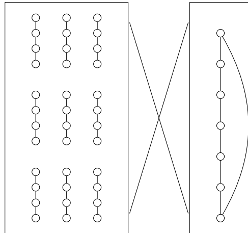
Figure 2: Example of G_{9,7} of Lemma 23
