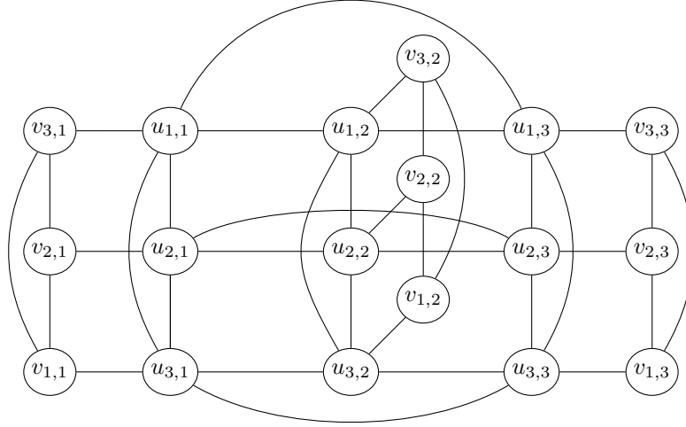
Figure 3: Example of graph G of Theorem 43 with t = k = 3 .
