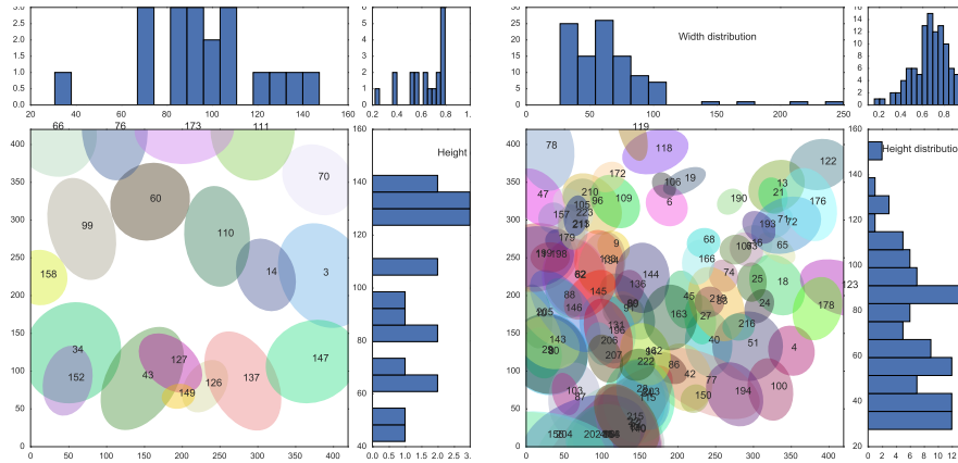
Figure 8: Characterizing cells using the checkerboard stimulus: Estimations of the Receptive Fields of representative retinal ganglion cells using a checkerboard stimulus. On the left we show the ON cells and on the right the OFF cells. The large plot is the map of the location of each receptive field. We show the ellipses corresponding to the best fits on the RFs' shapes. Adjacent to them are the histograms of the distribution of height and width, and in the corner is the distribution of the eccentricity of the ellipses fitted to the RF.
