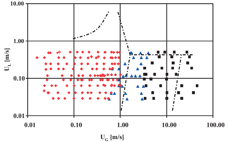
Figure 2. Flow regime map obtained for \text{N}_2 -ethanol flow in a glass capillary, d=400\mu\text{m} , adapted from [16]. Slug flow ( \blacklozenge ); slug-annular flow ( \blacktriangle ); annular flow ( \blacksquare ); flow transition lines from [13] (---).
