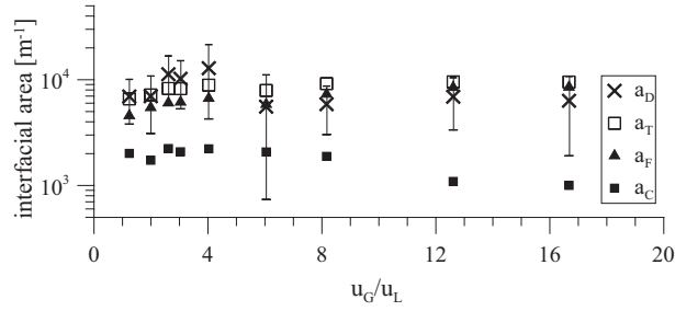
Figure 8. Comparison of interfacial area values obtained by Danckwerts' and photographic methods; error bars mean the 95 % confidence limits [53].
