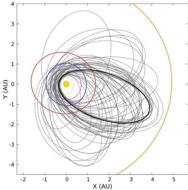
Figure 1. Projection on to the ecliptic plane of the current orbits of bodies in this study. The NEAs’ orbits are represented in grey, while 2P/Encke is drawn in black. The orbits of the planets from Mercury to Jupiter are plotted in colour.
