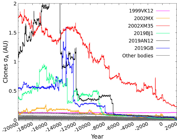
Figure 4. Standard deviation of the semimajor axis of the clones associated with various bodies as shown in the legend. One hundred clones were created for each body and integrated 22 000 yr in the past.
