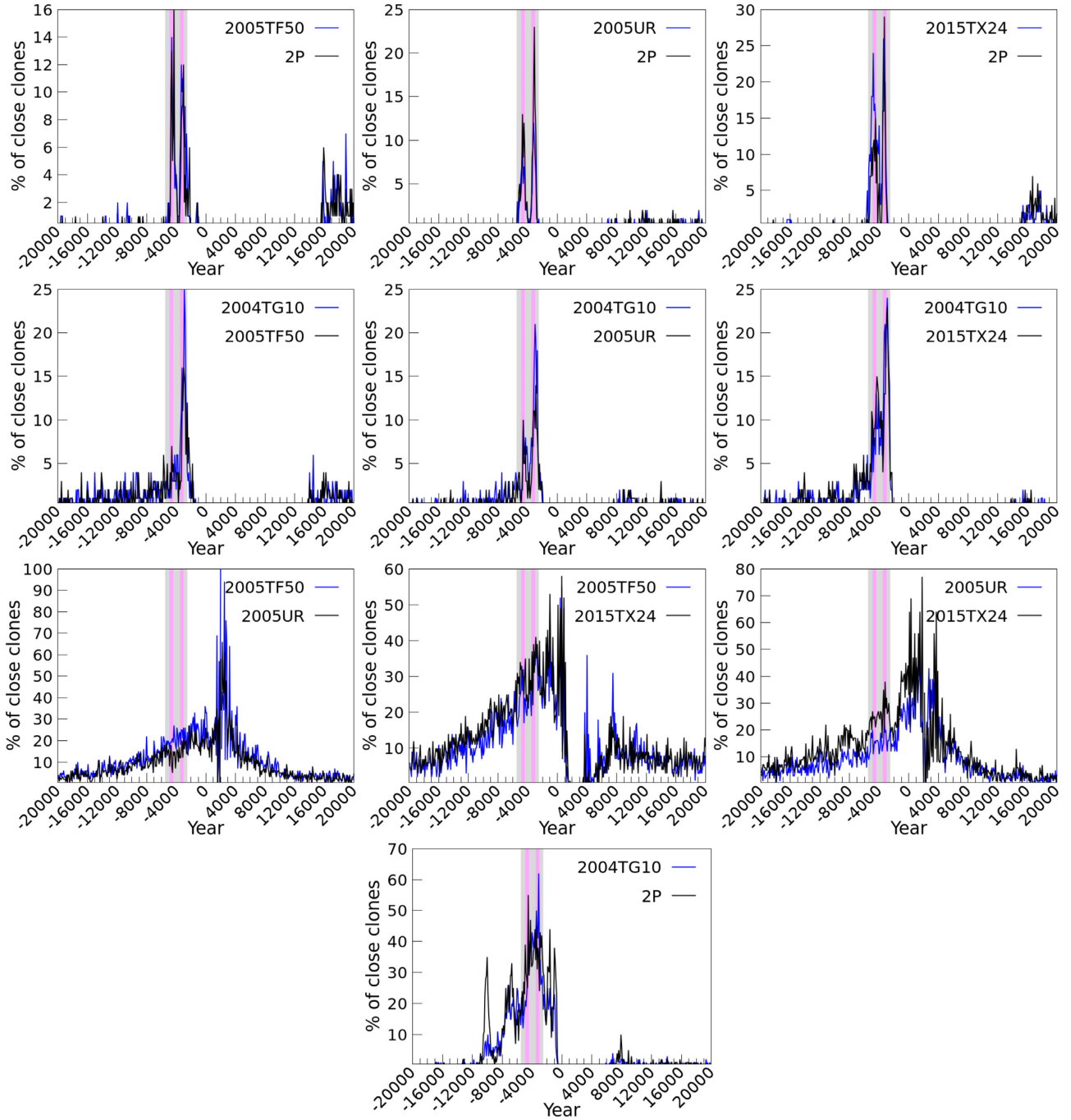
Figure 7. Percentage of clones of body #1 (in blue) and body #2 (in black) approaching at least a clone of the other object with a MOID smaller than 0.05 AU and a relative velocity below 500 m/s. The grey shaded areas encompass the period 2500 BCE to 5500 BCE, and the two magenta areas the years 3000 BCE to 3500 BCE and 4400 BCE to 4900 BCE, respectively.
