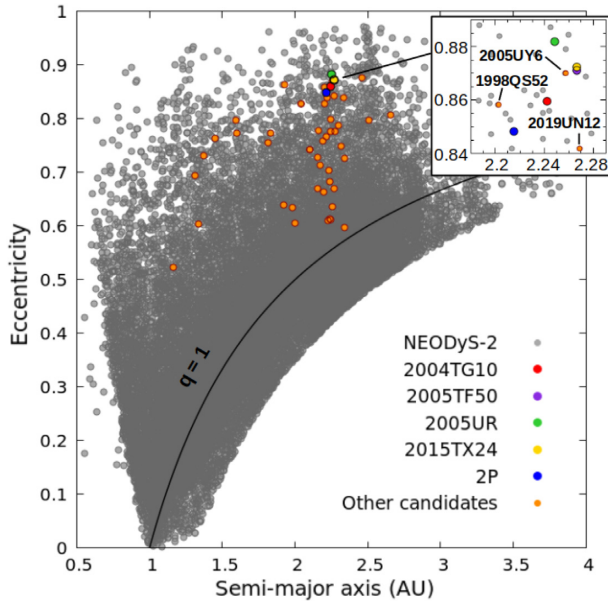
Figure 3. Semimajor axis and eccentricity of TC candidates (in colour) compared with all NEAs listed in the NEODyS-2 catalogue (in grey). The inset of the figure shows a small cluster of TC candidates with (a, e) orbital elements similar to comet 2P/Encke.
