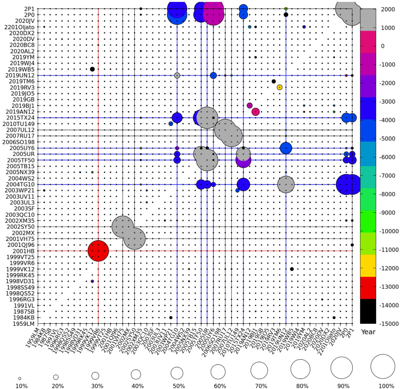
Figure 5. Possible rapprochements (close approaches) between osculating orbits of TC candidates over the period 20000 BC to 2000 CE. Labels on the abscissa and ordinate indicate the bodies integrated. Circles at position (body #1, body #2) indicate the percentage of clones of body #1 approaching at least one clone of body #2 with a MOID smaller than 0.05 AU and a relative velocity below 1 km/s. The size of the circle is proportional to the maximum percentage of clones retained for body #1 (in abscissa) compared to body #2 (in ordinate) over the integration period. The colour of the circle indicates the epoch when this highest percentage of clones retained is attained. The colour range has been restricted to the period 15000 BCE to 2000 CE for clarity. Coordinates with no rapprochements are still given a small black dot to help guide the eye in reading the figure.
