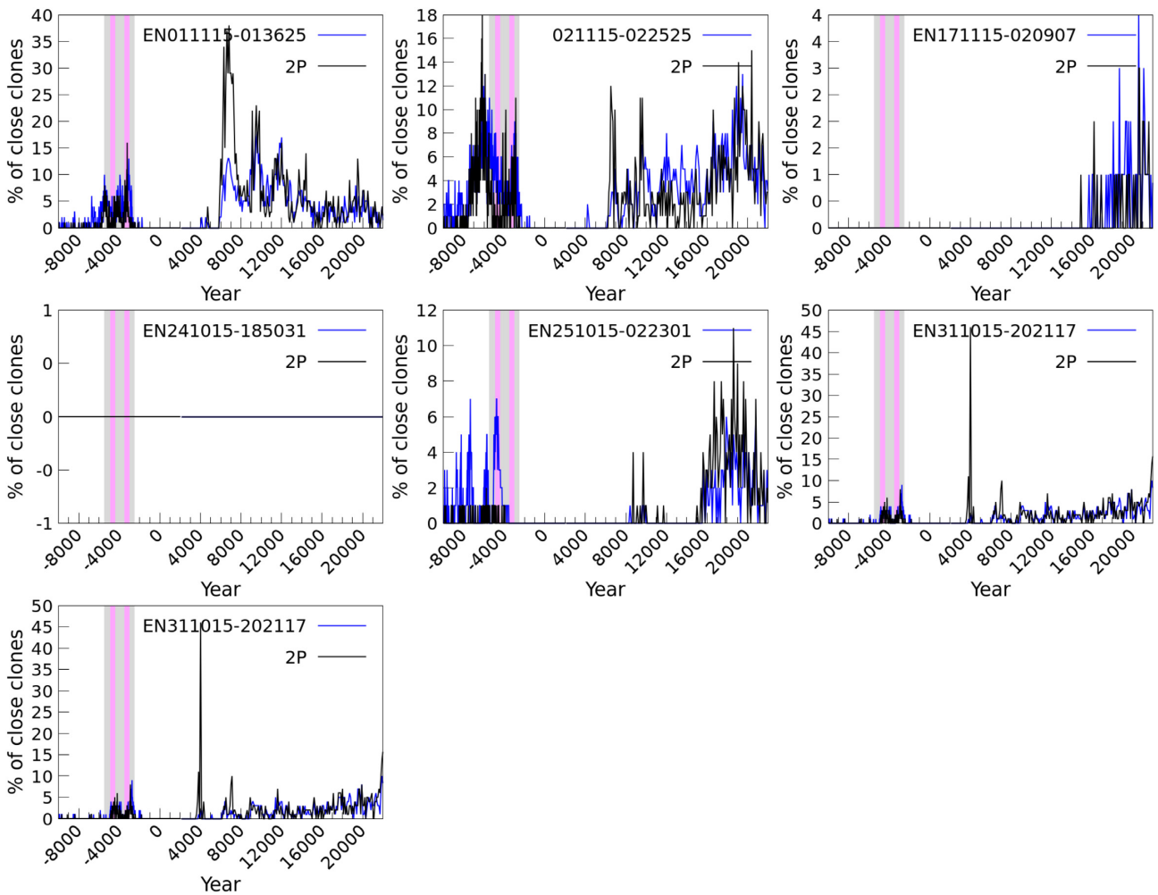
Figure 13. Percentage of the clones for each of the 2015 Taurid fireballs (in blue) and comet 2P/Encke (in black) approaching at least a clone of the other object with a MOID smaller than 0.05 AU and a relative velocity below 1 km/s. The grey shaded areas encompass the period 2500 BCE to 5500 BCE, and the two magenta areas the years 3000 BCE to 3500 BCE and 4400 BCE to 4900 BCE, respectively.
