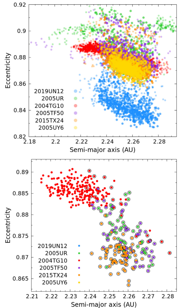
Figure 10. Semimajor axis and eccentricity of the clones created for 2004 TG10, 2005 TF50, 2005 UR, 2015 TX24, 2005 UY6, and 2019 UN12 between 3000 BCE and 3500 BCE (top). Particles trapped in the 7:2 MMR with Jupiter are indicated by a circled cross. In the bottom, only the clones approaching at least one clone of comet 2P/Encke within the threshold (MOID < 0.05 AU; V_r < 500 m/s) are represented. Resonant clones are circled in black.
