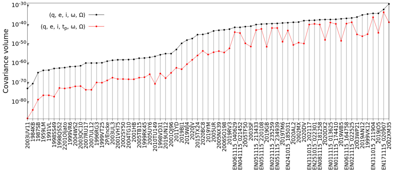
Figure 2. Volume of the hyperellipsoid of dimensions 5 and 6 defined by the variance–covariance matrix of the bodies integrated in \{e, q \text{ (AU)}, \Omega \text{ (}^\circ), \omega \text{ (}^\circ), i \text{ (}^\circ)\} (in black) and \{e, q \text{ (AU)}, t_p \text{ (d)}, \Omega \text{ (}^\circ), \omega \text{ (}^\circ), i \text{ (}^\circ)\} (in red).
