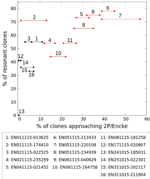
Figure 14. The percent of resonant clones for each of the 2015 Taurid fireballs as a function of the maximum percent of clones approaching 2P/Encke for each fireball retained during the close approach epoch around 3000 BCE. The range in percentage of clones retained for each body is represented by the line connecting the solid circles. The fireballs shown in Fig. 12 are highlighted in red.
