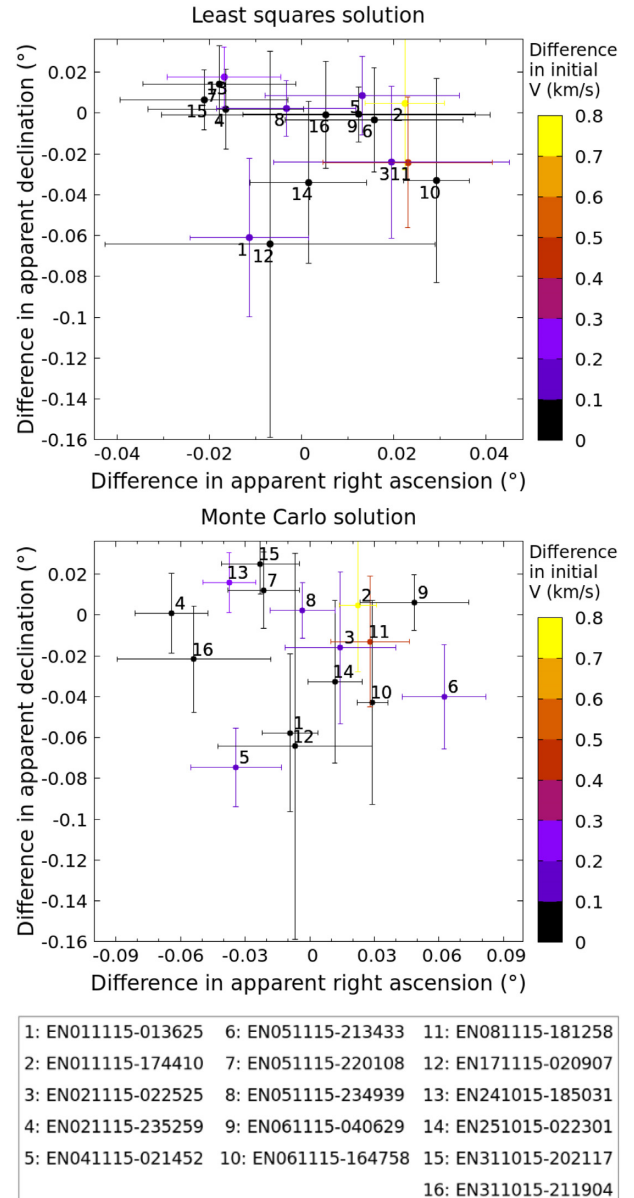
Figure 11. Difference in apparent radiant (right ascension and declination) and initial velocity (colour bar) of the fireballs state vectors computed with the line-of-sights method (top) or Monte Carlo solver (bottom) of the WMPL when compared with the EN solution. Each fireball is labelled by number and referenced by name following Table A2. See the text for details.
