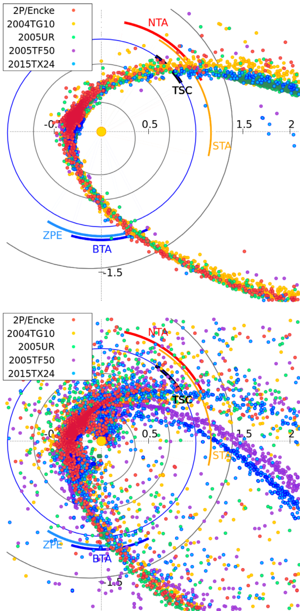
Figure 15. Distribution of nodal locations for model meteoroids crossing the ecliptic plane in 2015 based on ejection scenarios 2 (upper panel) and 3 (lower panel) for the G5 member’s orbit circa 3200 BCE (see text for details). The nodes are colour coded by the meteoroids’ parent body. The time periods where the annual Taurid meteor showers (NTA, STA, BTA, and ZPE) are active are indicated by the coloured arcs of circle close to the Earth’s orbit (in blue). The solar longitude range where the Taurid resonant swarm was observed in 2015 by Spurný et al. (2017) is illustrated by the black circle arc.
