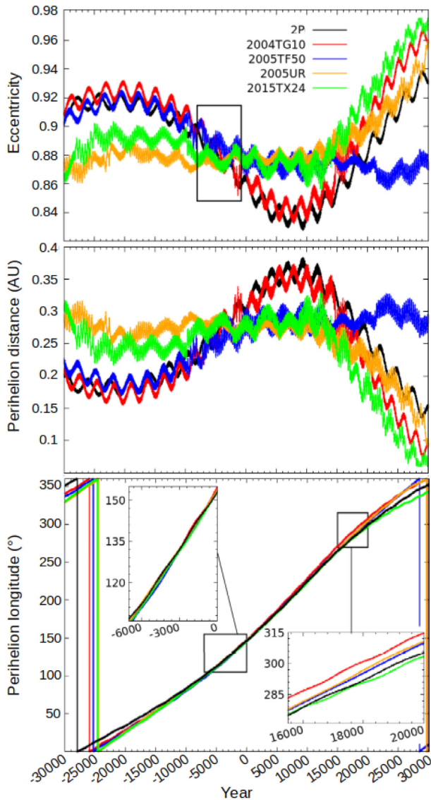
Figure 6. Eccentricity (top), perihelion distance (middle), and longitude of perihelion ( \varpi ) (bottom) evolution of the nominal clones created for 2P/Encke (in black), 2004 TG10 (in red), 2005 TF50 (in blue), 2005 UR (in orange), and 2015 TX24 (in green).
