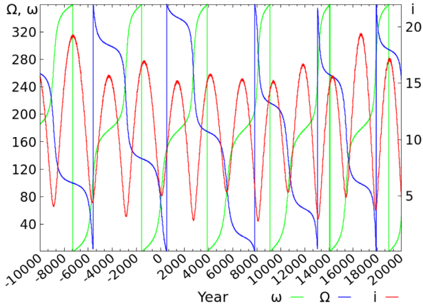
Figure 8. Inclination, argument of perihelion, and the longitude of the ascending node of comet 2P/Encke, integrated from the nominal solution of Table A1 without non-gravitational forces.
