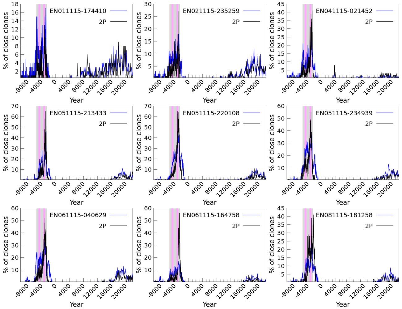
Figure 12. Percentage of the clones for each of the 2015 Taurid fireballs (in blue) and comet 2P/Encke (in black) approaching at least one clone of the other object with a MOID smaller than 0.05 AU and a relative velocity below 1 km/s. The grey shaded areas encompass the period 2500 BCE to 5500 BCE, and the two magenta areas bracket the years 3000 BCE to 3500 BCE and 4400 BCE to 4900 BCE, respectively.
