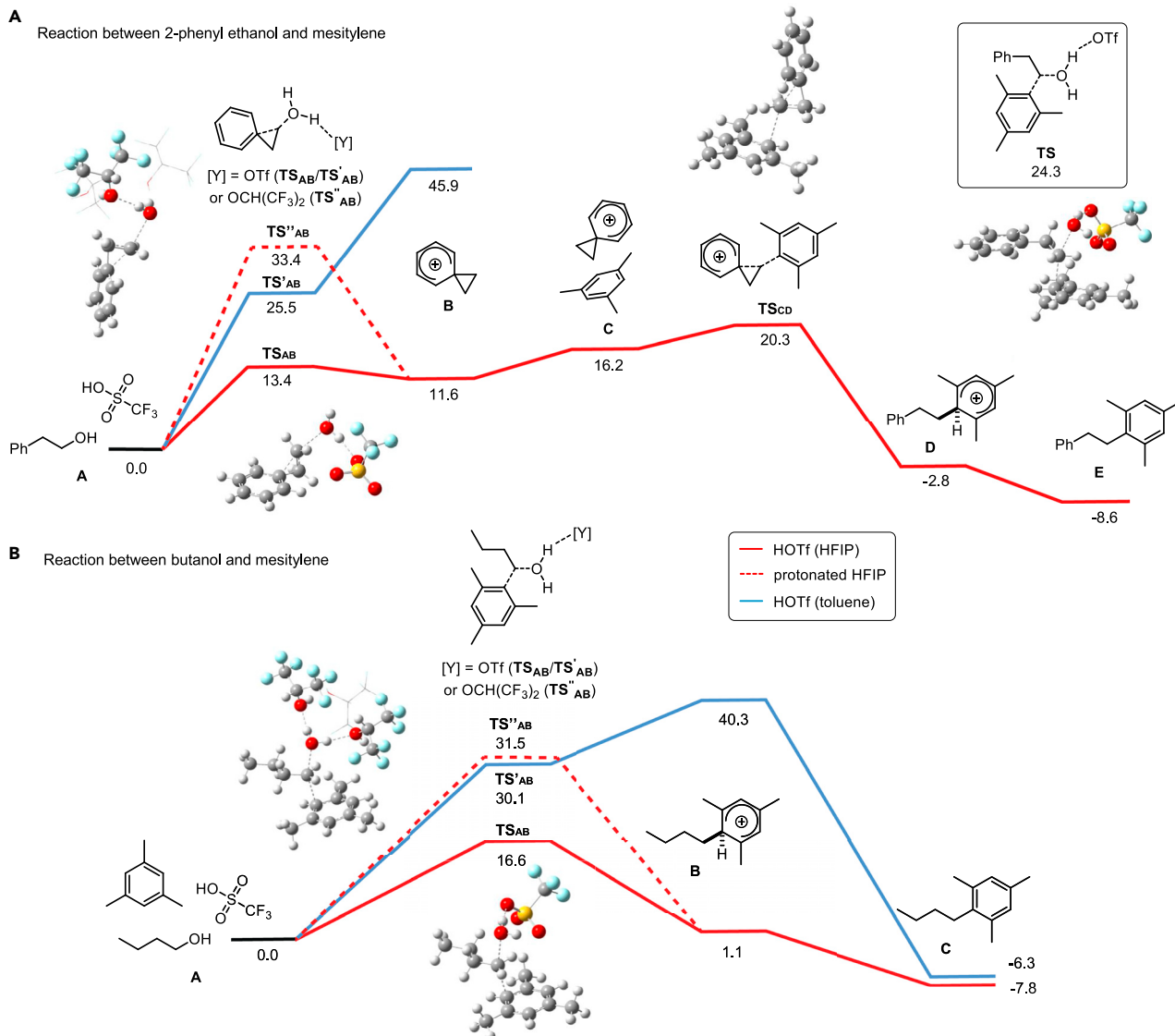
Scheme 6. Gibbs energy profiles ( \Delta G , kcal mol -1 ) for the addition of mesitylene to phenyl ethanol and to butanol
