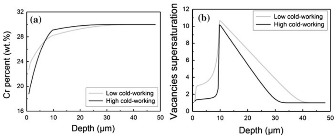
Fig. 6 Comparison of the Ni–30Cr alloy evolution for HCW case and the LCW case for 5 h oxidation at 1,273 K. a Cr depletion profiles and b vacancies concentration profiles
