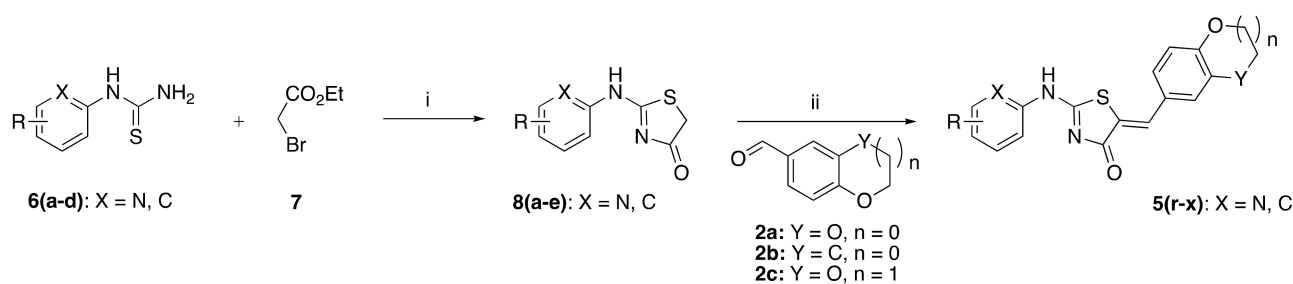
Scheme 2. General synthetic approach for the (5 Z ) 2- N -heteroaryl-amino-5-arylidene-1,3-thiazolidin-4-one derivatives 5r–x from the starting 2- N -heteroaryl-amino-1,3-thiazolidin-4-one 8a–e and aromatic aldehydes 2a–c . Reagents and reaction conditions: (i) 7 1.3 eq, EtOH, 55 °C, 3.5–22 h; (ii) piperidine 0.1 eq or AcONa 0.1 eq, AcOH 0.1–6.6 eq, 120–150 °C, MWI in closed vessel (Explorer 24 ® CEM \mu Wave reactor), 20–40 min.
