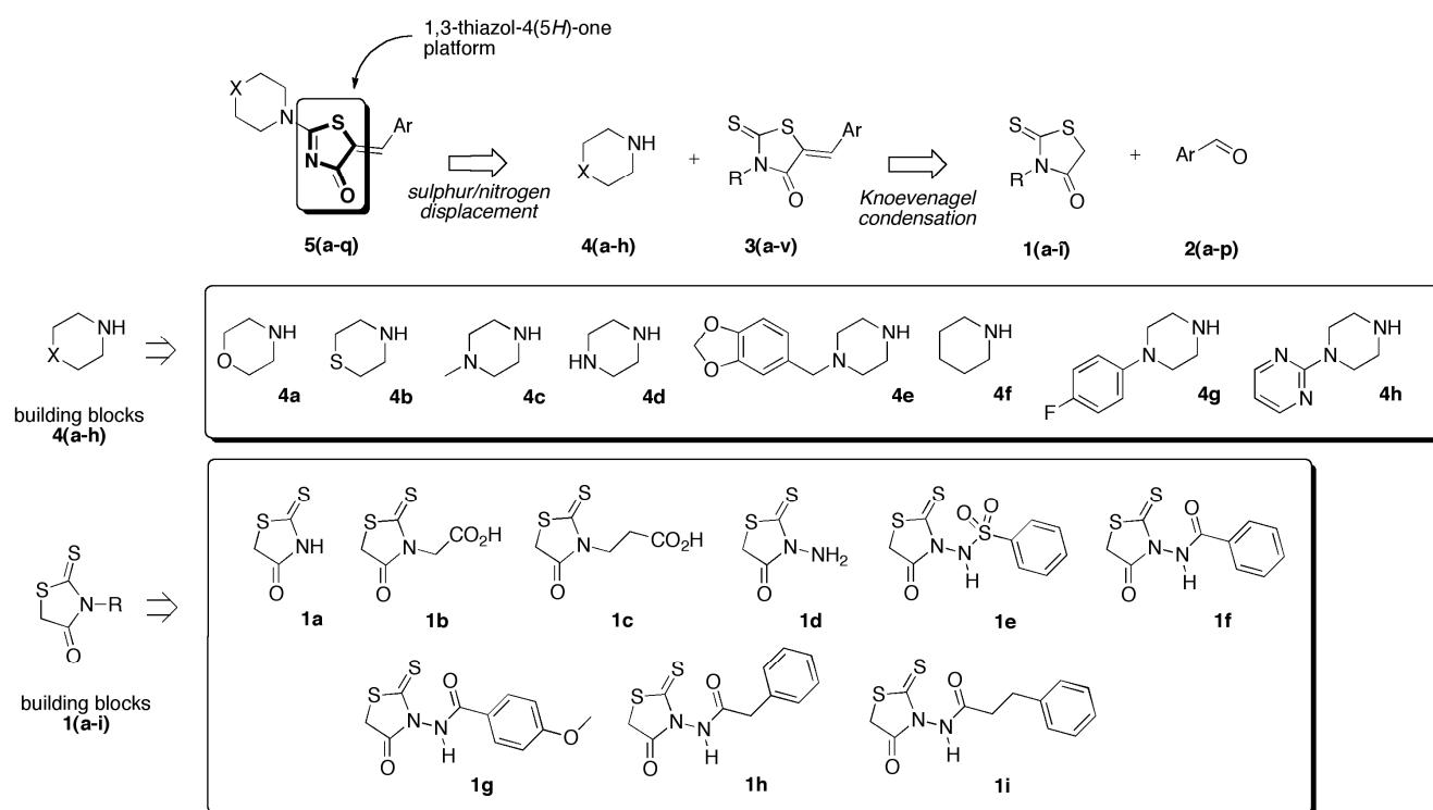
Figure 2. Retrosynthetic strategy toward new (5Z) 2-amino-5-arylidene-1,3-thiazol-4(5H)-ones 5a–q based on the use of secondary cyclic amines building blocks 4a–h in sulfur/nitrogen displacement reaction and the use of various 2-thioxo-1,3-thiazolidin-4-ones 1a–i as starting platforms in Knoevenagel condensation.
