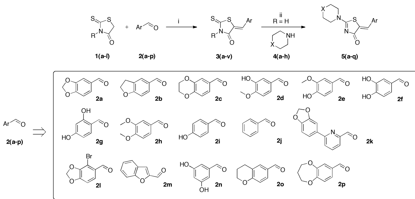
Scheme 1. General synthetic approach for the (5 Z ) 5-arylidene-2-thioxo-1,3-thiazolidin-4-one derivatives 3(a–v) and for the (5 Z ) 2-amino-5-arylidene-1,3-thiazol-4(5 H )-one 5a–q . Reagents and reaction conditions: (i) n -PrNH 2 2 eq, 80 °C, 30 min for compounds 3a–l in open vessel using Synthewave ® 402 reactor for MWI; Et 3 N 0.1 eq or piperidine 0.1 eq or AcONa 1 eq, AcOH 0.1–6.6 eq, 85–150 °C, 20–210 min for compounds 3m–v in closed vessel using Explorer 24 ® CEM or Monowave ® 300 Anton-Paar reactors for MWI. (ii) 4a–h 1.2 eq, MWI in Synthewave ® 402 microwave reactor, 80 °C, 20–60 min.
