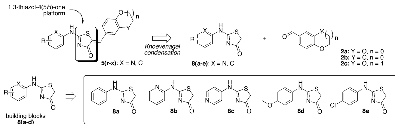
Figure 3. Retrosynthetic strategy toward new (5Z) 2-N-heteroarylamino-5-arylidene-1,3-thiazol-4(5H)-ones 5r–x based on the use of aromatic aldehydes 2a–c and various 2-N-heteroarylamino-1,3-thiazolidin-4-one 8a–e as other starting platforms in Knoevenagel condensations.
