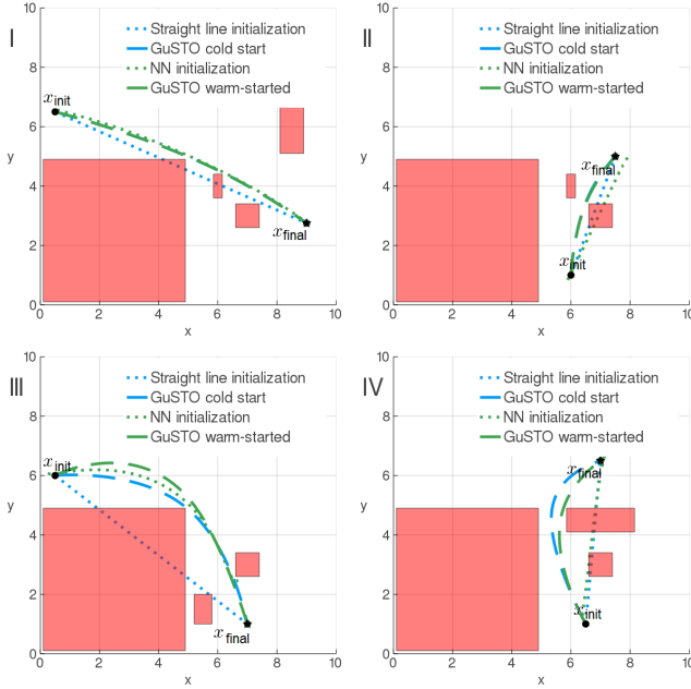
Figure 5: Trajectory optimization results in presence of obstacles which are not in the training set of the neural network. Although the prediction is often infeasible, the neural network can still be used to warm-start GuSTO, reducing computation time and leading to a feasible solution for OCP .
