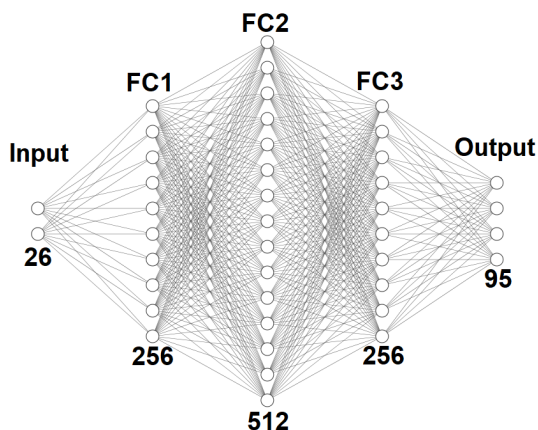
Figure 2: Architecture of the neural network predicting an initializing strategy for GuSTO. ReLU activation functions are used for each neuron.
