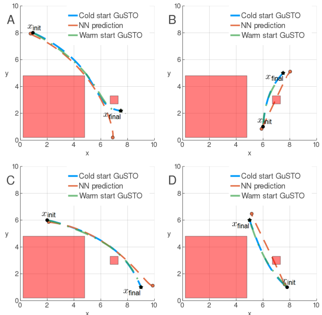
Figure 4: Four scenarios comparing the trajectories obtained from (1) GuSTO initialized with a straight line, (2) direct inference from the neural network, and (3) GuSTO warm-started with the neural network prediction.
