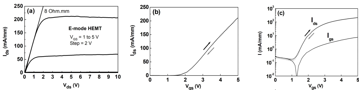
Figure 4. (a) DC output characteristics of a 1.5 μm gate E-mode transistor. (b) Hysteresis transfer characteristics V_{ds} = 7\text{V} . Solid line shows I_{ds} for positive sweep of the gate bias; dashed line represents
