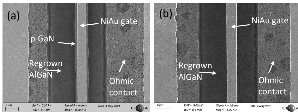
Figure 2. Scanning electron microscope views of the (a) E-mode and (b) D-mode transistors.
