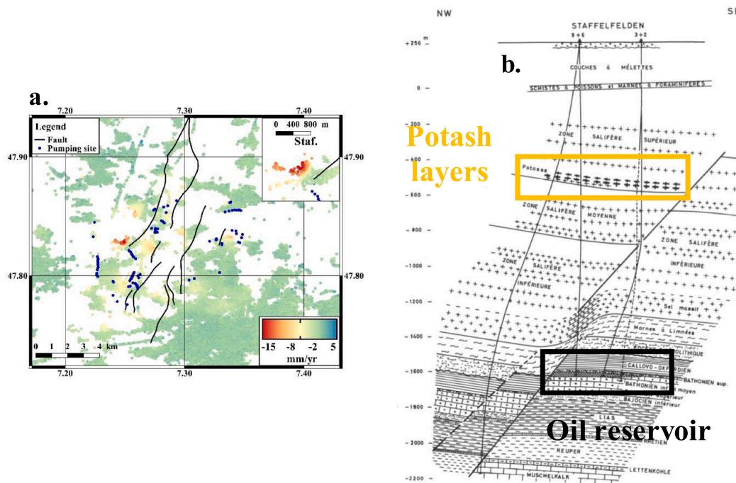
Fig. 7. Potential sources of surface displacements. a: Mean LOS velocity during ENVISAT period with the pumping sites (blue circles) and faults (black lines); b. Geological section across Staffelfelden (adapted from Sittler, 1972). The location of faults at depth has been projected at the surface. (For interpretation of the references to color in this figure legend, the reader is referred to the web version of this article.)
