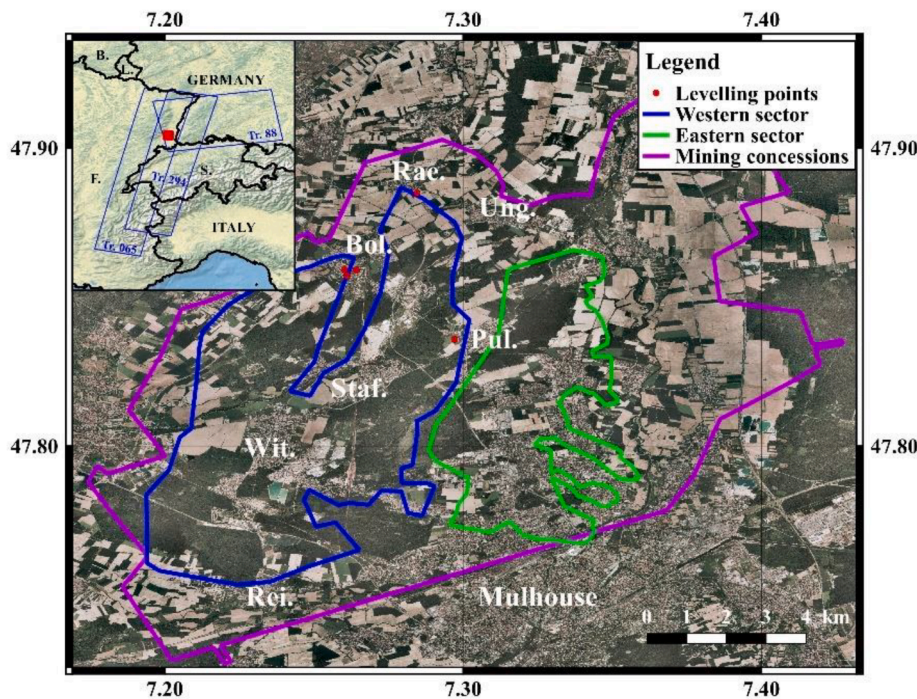
Fig. 2. Map of the Alsatian potassic basin. The background is the IGN orthophotography (2002). Bol.: Bollwiller, Pul.: Pulversheim, Rae.: Raedersheim, Rei.: Reiningue, Staf.: Staffelfelden, Wit.: Wittelsheim, Ung.: Ungersheim. Inset: Location of the MDPA (red square) at the regional scale. Blue rectangles represent the coverage of each track of SAR images. B.: Belgium, L.: Luxembourg, F.: France, S.: Switzerland. (For interpretation of the references to color in this figure legend, the reader is referred to the web version of this article.)
