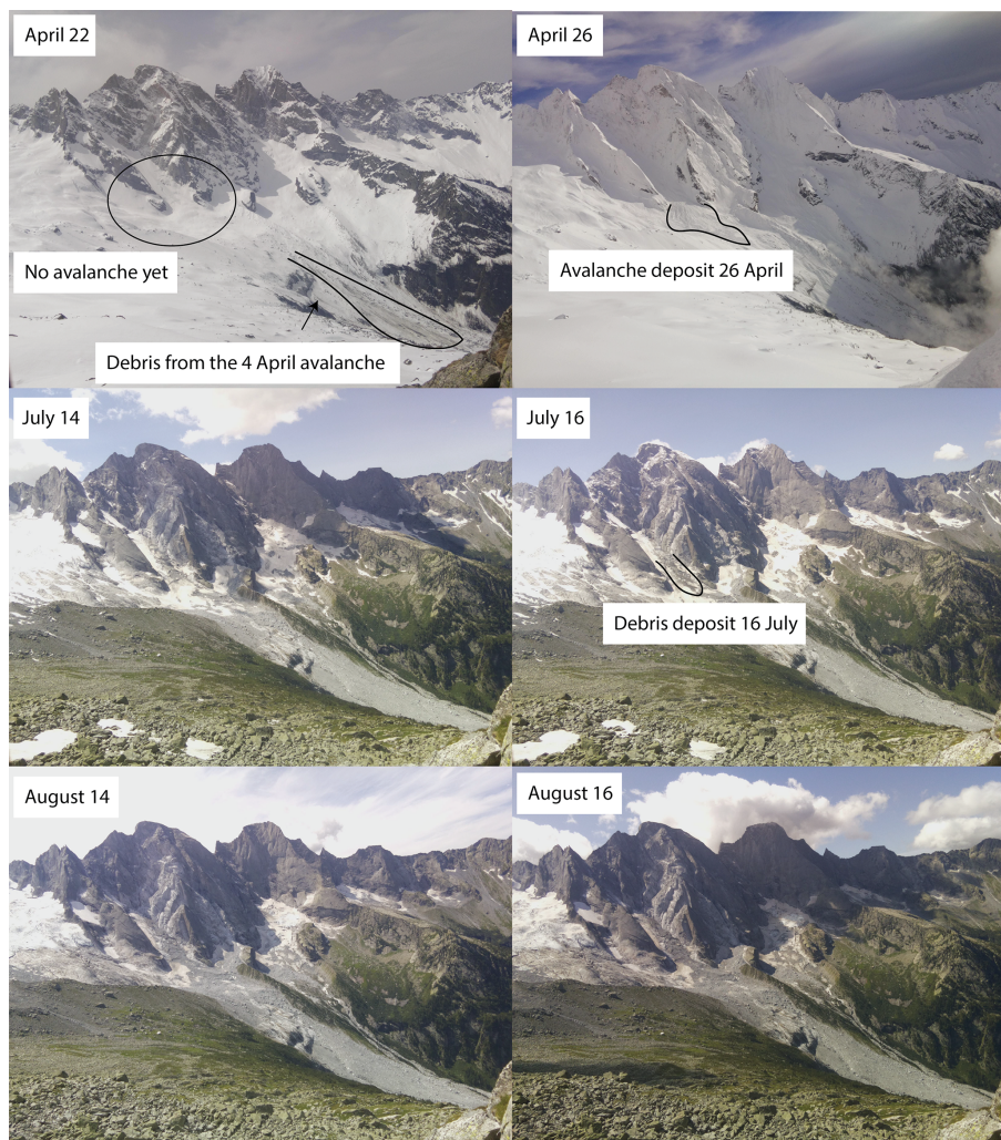
Figure 8. Automatic-camera photos of slope failures in 2019. Photos from April show the avalanche deposits from the events classified as slope failures of 4 and 26 April. Photos from July and August are from before and after the events of 16 July and 14 August. For the 14 August event, no deposit is visible on the photos.
