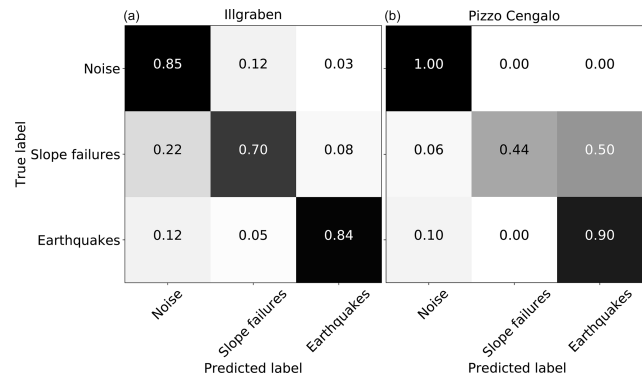
Figure 5. Confusion matrices of an initial test of the continuous random forest approach on 20 s windowed data. (a) Illgraben data set, (b) Pizzo Cengalo data set.
