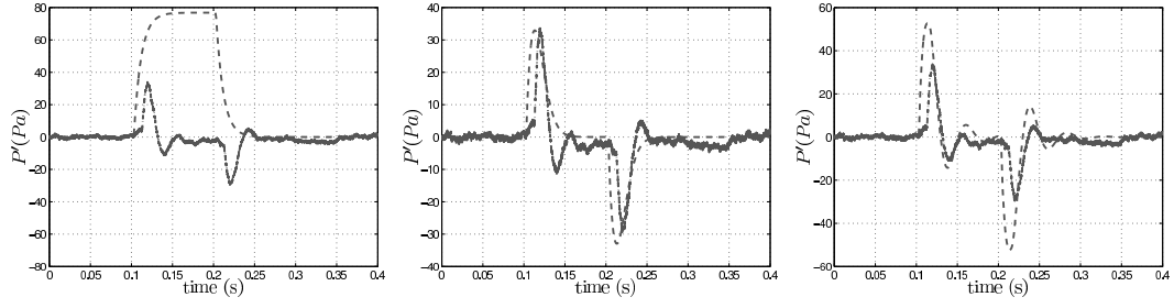
(a) Non-reflecting inlet ( R_1 = 0 ) and outlet ( R_2 = 0 ) (b) Non-reflecting inlet ( R_1 = 0 ) and partially reflecting outlet (c) Reflecting inlet and outlet
